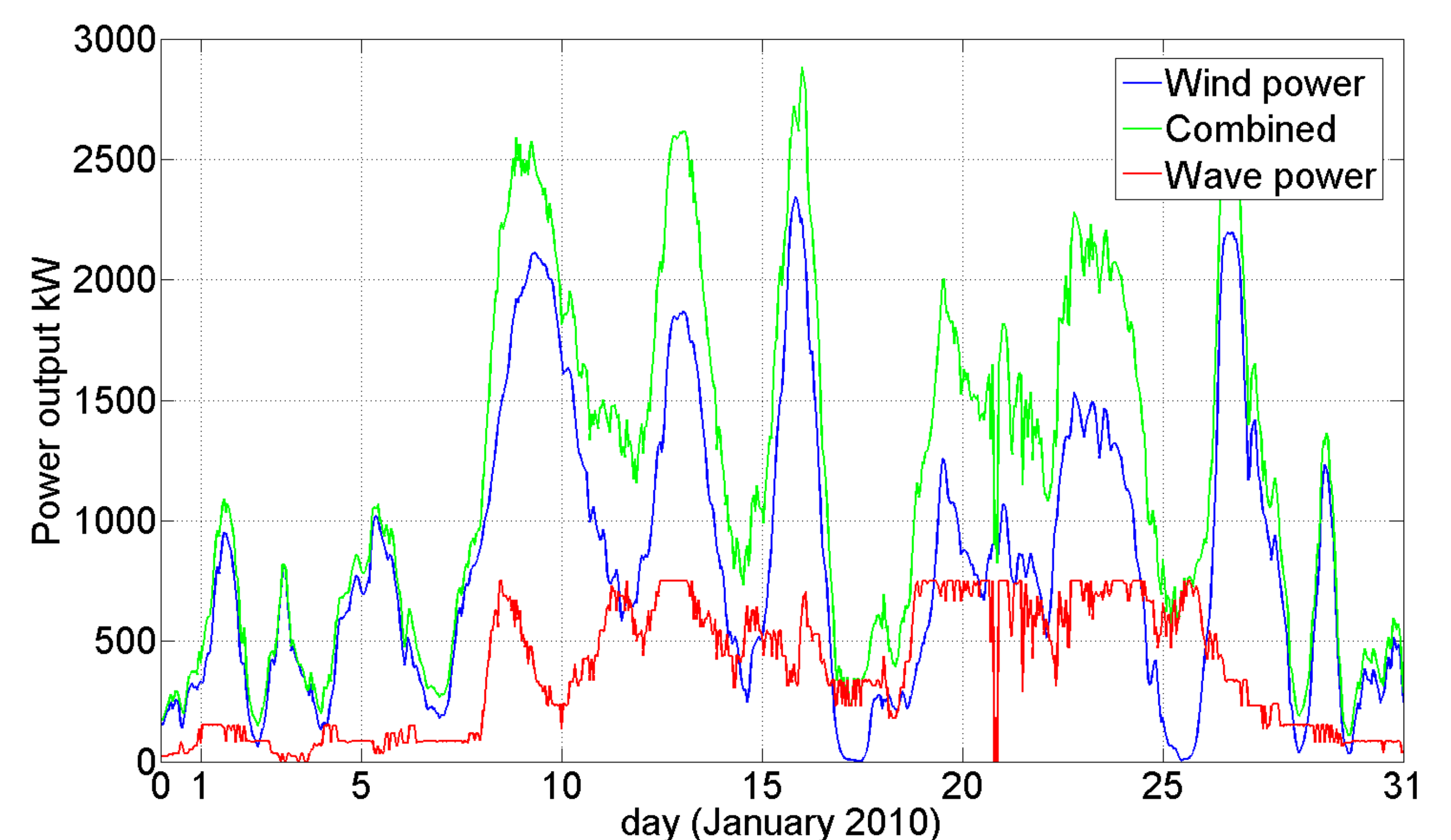
Fig. 2 The power output from the wind turbine and wave device
