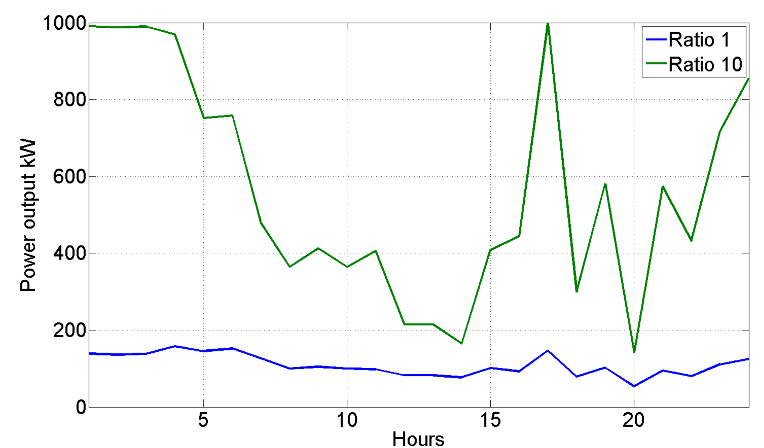
Fig. 3 Simulated power output from wind and wave integration
