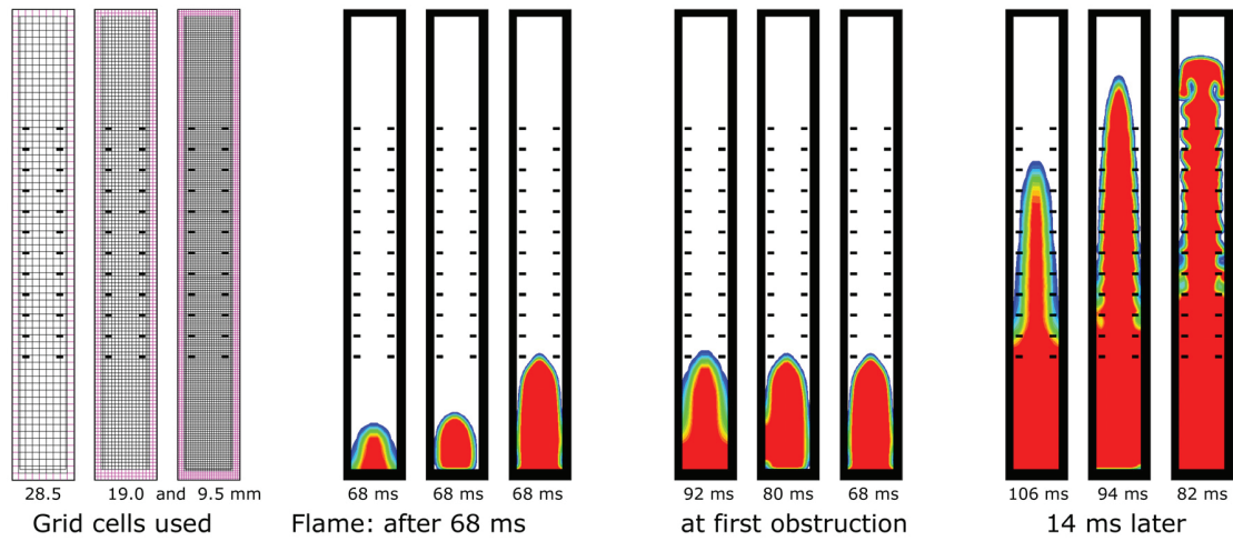
Figure 5 Vertical cross-section of simulated pipe, illustrating grid cells and simulated flame development for various grids during a cornstarch-air explosion. Flames are plotted as mass fraction of combustion products at various time-steps: after 68 ms, when the flames reaches the first obstruction, and 14 ms after the flames reached the first obstruction. The modelled cornstarch had a K_{St} value of about 150 bar m/s.
