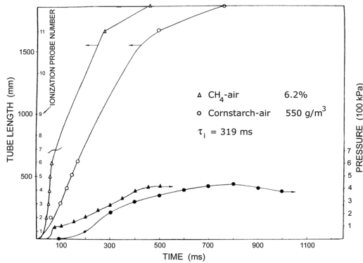
Figure 2 Pressure rise and location of flame front as functions of time in 1.86 meter closed tube for mixtures of 6.2 % methane in air and 550 g/m 3 cornstarch in air (from Pu, 1988).
