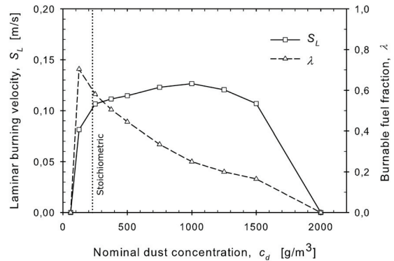
Figure 4 Laminar burning velocity and fraction of burnable fuel used as input to DESC; lower flammability limit estimated to 60 g/m 3 , upper flammability limit arbitrary set to 2000 g/m 3 .
