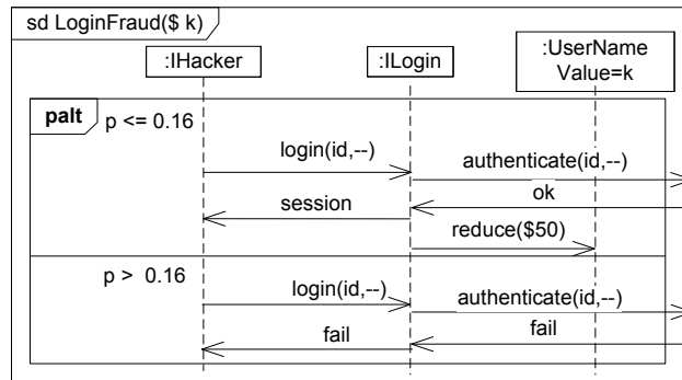
Fig. 5. Login without password using SQL injection
