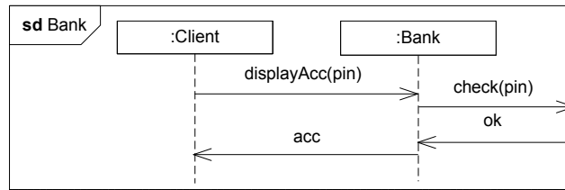
Fig. 3. Example interaction
