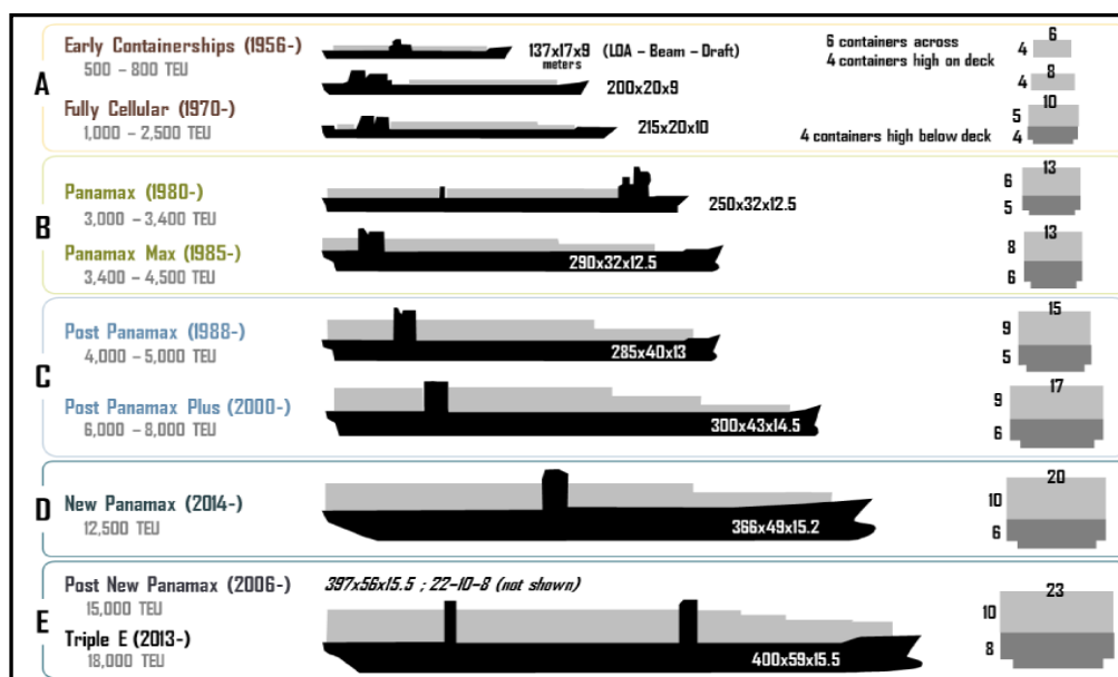
Figure 1.2- Evolution of container ships
