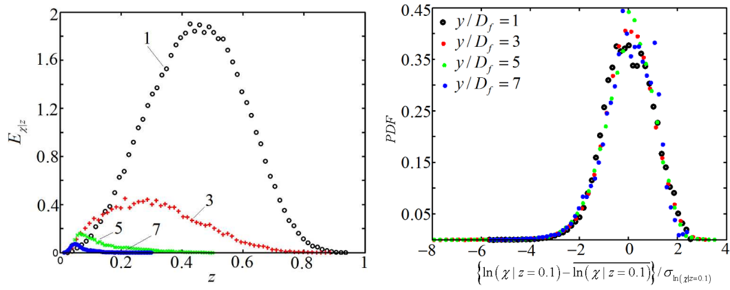
Figure 4.79: Weighted probability of occurrence of the mean conditional scalar dissipation rate (left) and conditional p.d.f. \left[ \ln(\chi|z=0.1) - \overline{\ln(\chi|z=0.1)} \right] / \sigma_{\ln(\chi|z=0.1)} (right) for S = 1.07 at y/D_f = 1, 3, 5, 7 computed from window 2.
