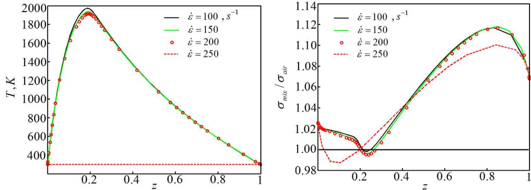
Figure 2.12: Temperature as a function of mixture fraction (left) and the ratio of Rayleigh scattering cross section of the mixture to the air (right), obtained from opposite–flow simulation for DLR fuel as a function of strain rate (1/s). Temperatures of fuel and oxidiser were 300(K) and GRI-3.0 detailed chemical mechanism was used. Strain rate varied from 100 to 250 (1/s), where for 250 (1/s) extinction was observed.
