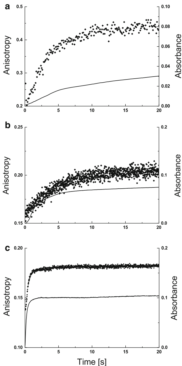
Fig. 1 Fluorescence anisotropy at 280 nm ( diamond ) and absorbance at 320 nm ( solid line ) of cytochrome C in 8 M urea refolded at 1:5 (a), 1:10 (b) and 1:25 (c) by dilution with 100 mM TRIS pH 10.6, to a final protein concentration of 6.4 \times 10^{-5} M
