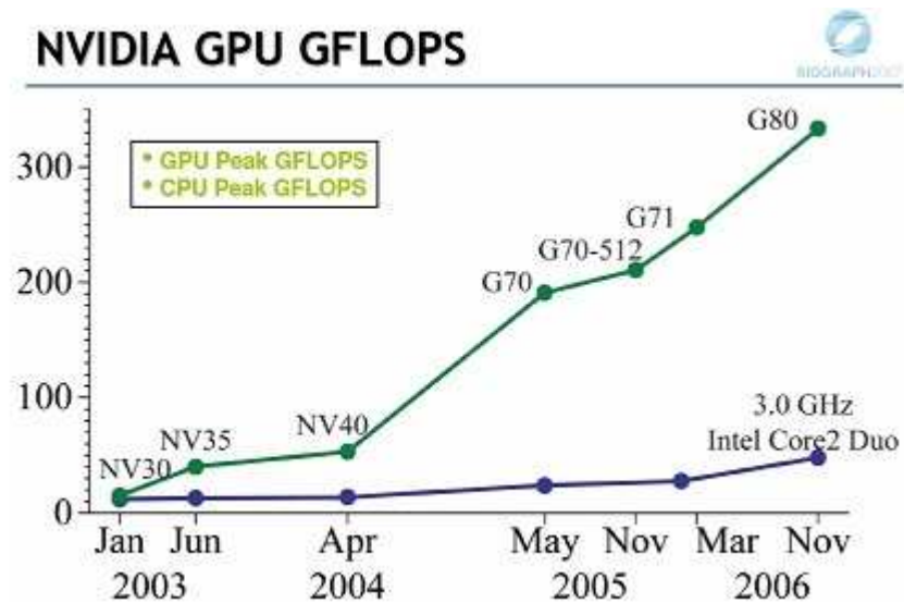
Figure 9: gigaFLOPS comparison (Green, 2007)
