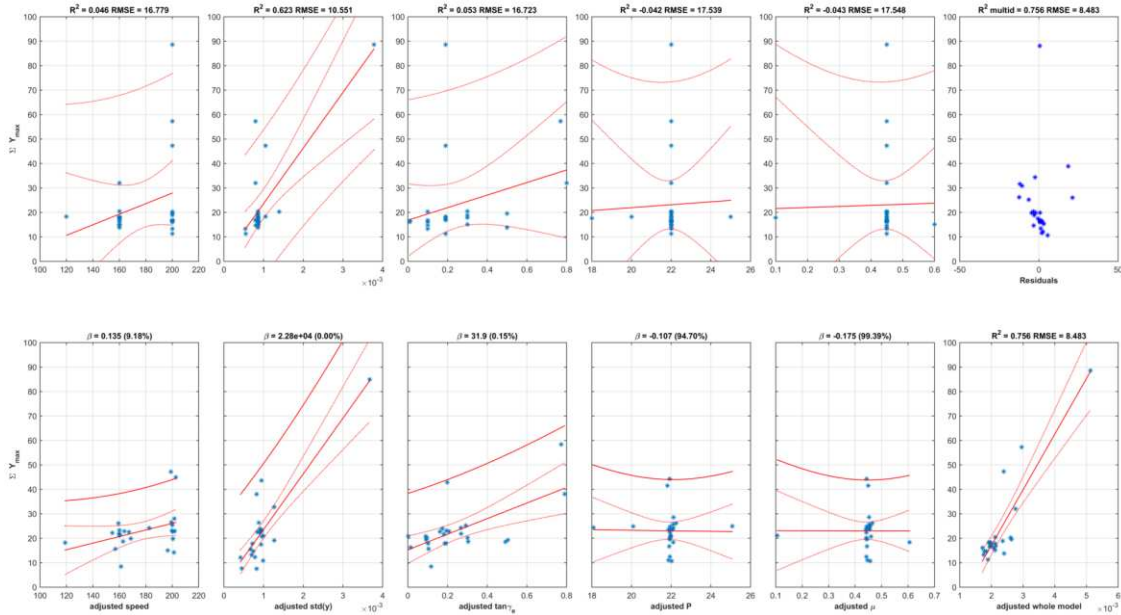
Figure 11: Parameters affecting \sum Y_{\max} for the BB26000 locomotive on straight track, plots with: speed; track geometry standard deviation (lateral); equivalent conicity ( \tan \gamma_e ); axleload (P); wheel-rail friction ( \mu )
