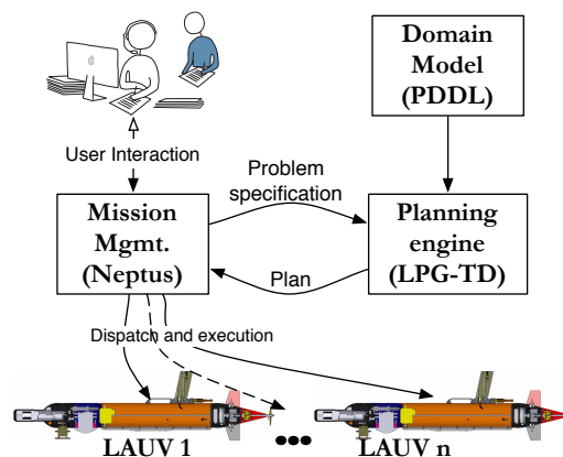
Fig. 2. A modular architecture of the system. deals with a problem of finding a sequence of actions that transform the environment from a given initial state to a desired goal state [16]. The simplest form of automated planning works in deterministic, fully observable and static environment, where effects of actions are instantaneous. Temporal planning, which is the focus of our interest, allows “durative actions” whose planning and execution makes explicit use of, and reasons with, the notion of time.
