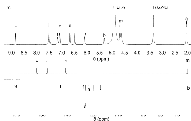
Fig. 4. 1 H and 13 C[ 1 H]. NMR spectra of \Lambda_{\text{Fe}}[\text{Fe}_2\text{L}^{2e_3}]\text{Cl}_4 \cdot 9\text{H}_2\text{O} at 298 K in d 4 -methanol; see Fig. 2 for key.
