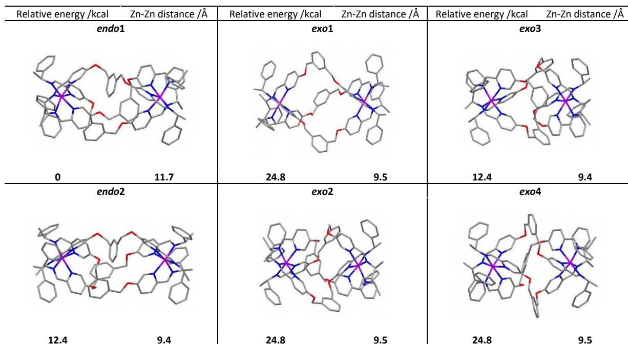
Fig. 3. DFT Calculated structures, relative energies (compared to endo1 ) and Zn-Zn distances of the six conformational isomers of \Lambda_{Zn}[\text{Zn}_2\text{L}^{2e_3}][\text{ClO}_4]_4 . d) Linear decay of \ln(\epsilon) at 540 nm (corresponding to MLCT band) of [\text{Fe}_2\text{L}^{2e_3}]\text{Cl}_4 (0.03 mM in 0.2 M HCl).
