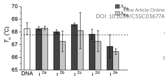
Fig. 7. Effect on T_m of linear ct-DNA (DNA, white) from interactions [\text{Fe}_2\text{L}^n_3]\text{Cl}_4 ( n = 2a-2e ) ( \Delta_{\text{Fe}} - light grey, \Lambda_{\text{Fe}} - dark grey) in 1mM Trizma base (10 base pairs of DNA to 1 flexicate complex).
