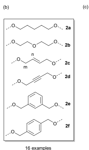
Fig. 2. (a) Synthesis of new flexicates; (b) linking groups used in this study; (c) Sections of 1 H NMR spectra of \Lambda_{Zn} - [Zn_2 L^{2e_3}][ClO_4]_4 \cdot 4.4H_2O at 253 – 353 K in d 2 -acetonitrile showing the higher equilibrium population of a minor asymmetric conformer at higher temperatures.
