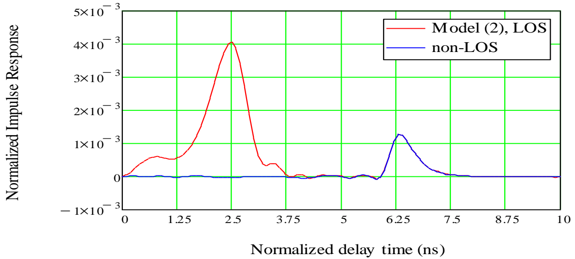
Figure 7-11-VLC channel response
