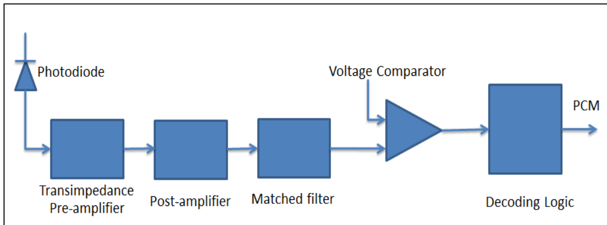
Figure 9-3-Optical receiver
