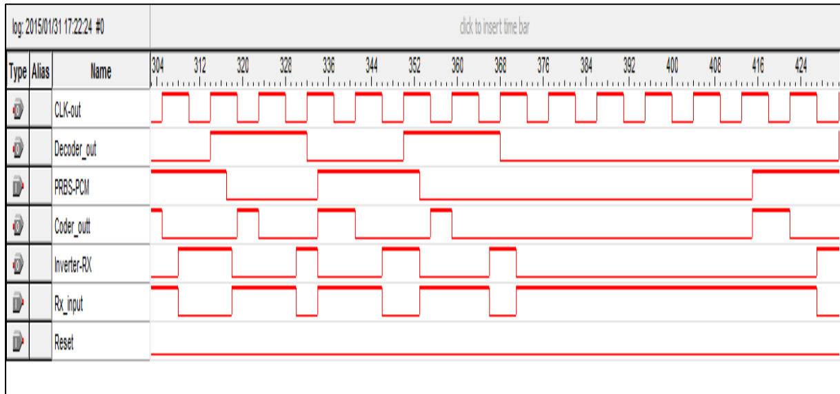
Figure 9-10-DiPPM System results
