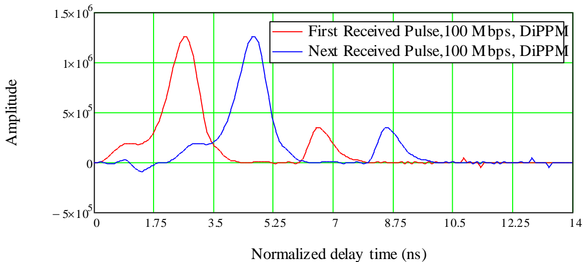
Figure 7-15 Response of DiPPM with zero guards
