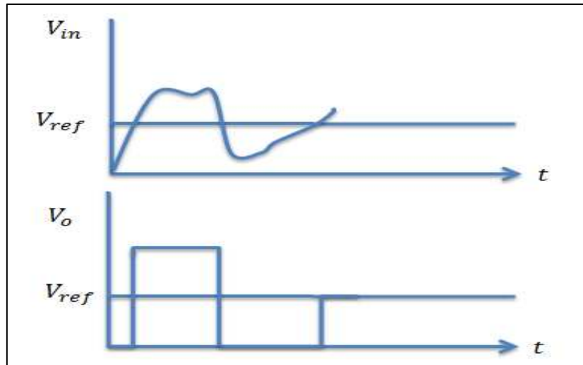
Figure 9-5-Comparator Input/Output
