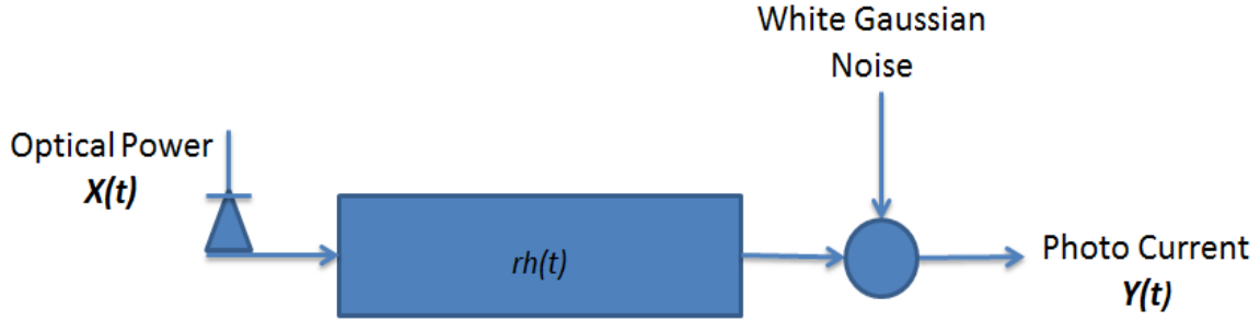
Figure 4-2-Optical Wireless Channel
