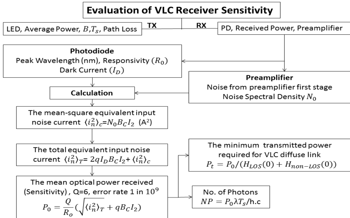
Figure 8-2-Receiver Sensitivity Determination
