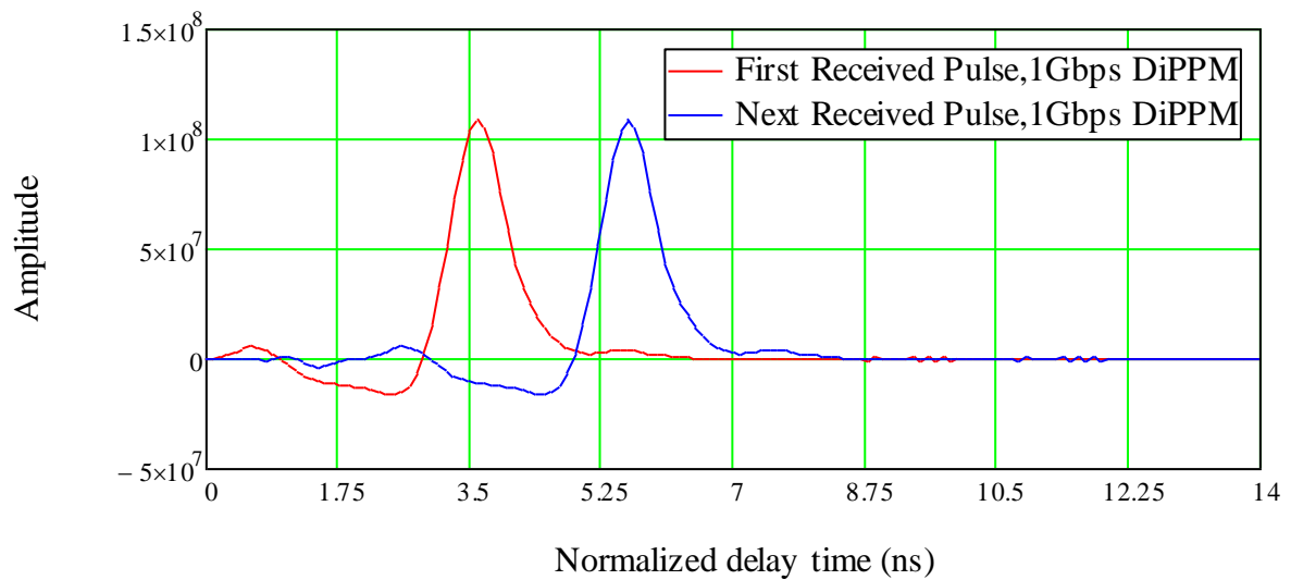
Figure 7-6-Response of DiPPM with two guards
