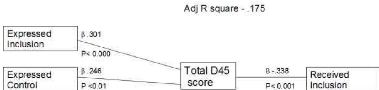
Figure 8.9 Path model of FIRO-B elements predicting level of D45.
