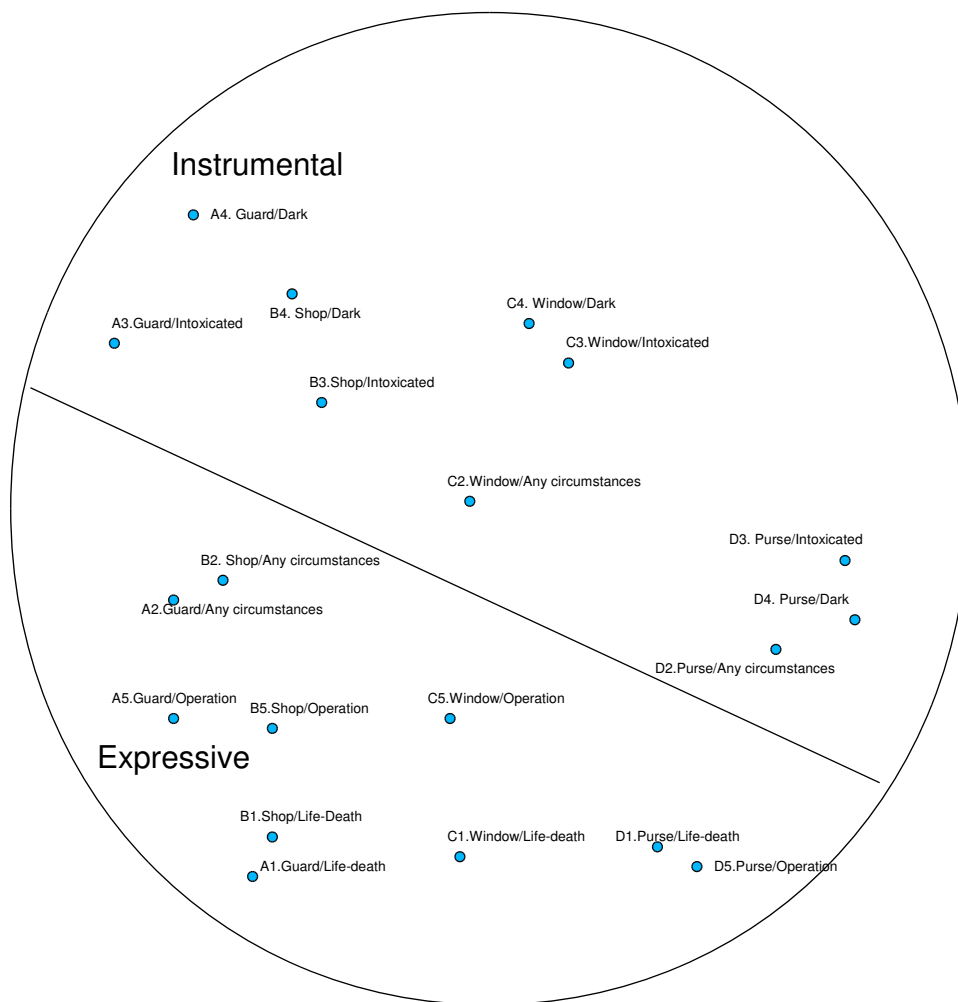
Figure 5.11 SSA plot showing structure of items defining justification styles.
