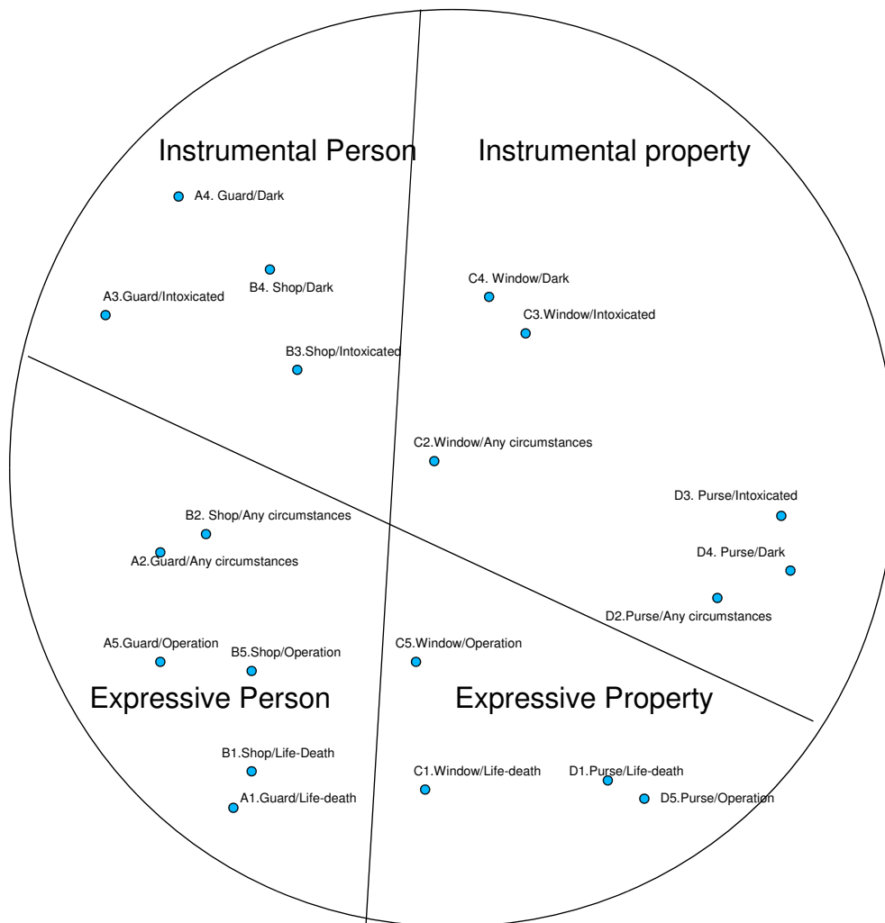
Figure 5.12 SSA plot defining both crime scenario and justification styles.
