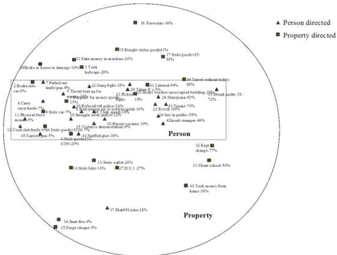
Figure 7.5 SSA plot showing structure of items representing form of interaction
