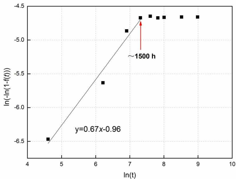
Fig.11 Evaluation of time exponent n based on the quantification results of the area fraction of Laves-phase precipitates in P92 steel at 923 K
