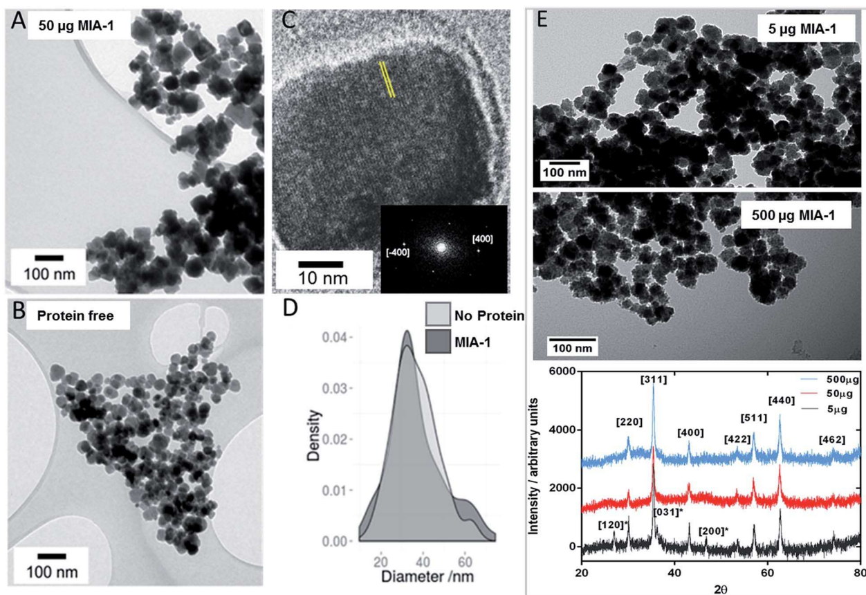
Fig. 7 Transmission Electron Microscopy analysis of magnetite nanoparticles. (A) Particles prepared with MIA-1 at 50 \mu\text{g} per 10 ml reaction. (B) Particles prepared in the absence of MIA-1. (C) HRTEM analysis of a representative MIA-1 prepared MNP. A region of the lattice fringe is highlighted with yellow lines and the Fourier transform is shown inset with the [400] peaks identified. (D) Particle size analysis of MNP prepared with and without addition of MIA-1. (E) Transmission Electron Microscopy and X-ray diffraction analysis of magnetite nanoparticles at varying amounts of MIA-1. Powder XRD analysis of particles produced at 5 \mu\text{g} (grey), 50 \mu\text{g} (red) and 500 \mu\text{g} (blue) of MIA-1. Principal magnetite peaks have been assigned. Peaks present in the 5 \mu\text{g} sample assigned to lepidocrosite are denoted with an asterisk.
