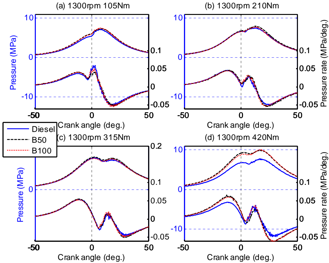
Figure 5. The variation of cylinder pressure and pressure rising rate
