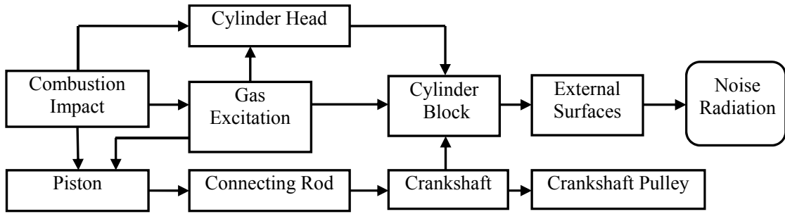
Figure 2. The combustion noise generation diagram
