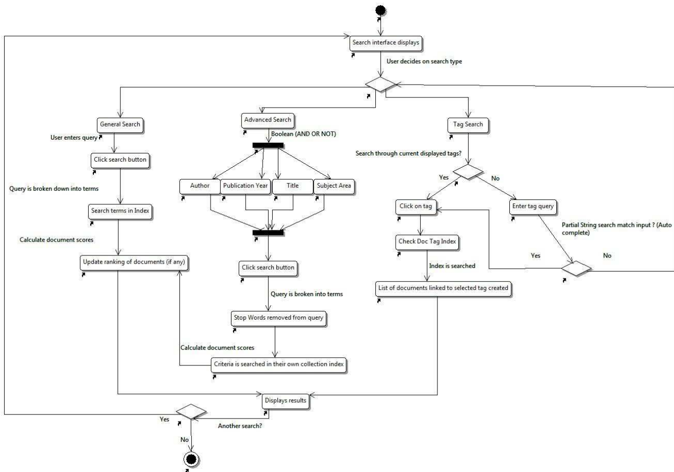
Fig. 9 Activity Diagram
