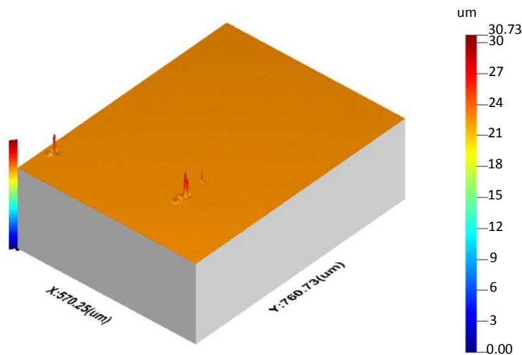
Figure 8: PET film areal measurement using WSI
