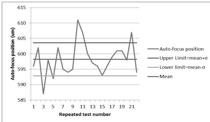
Figure 5: The repeatability of the auto-focus system
