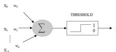
Fig. 1 Simple perceptron diagram
