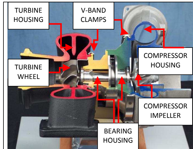
Figure 3 Turbocharger structural problems areas
