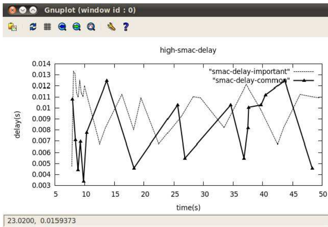
Figure 7-40 System Delay of the high-load S-MAC protocol in the Different Transactions
