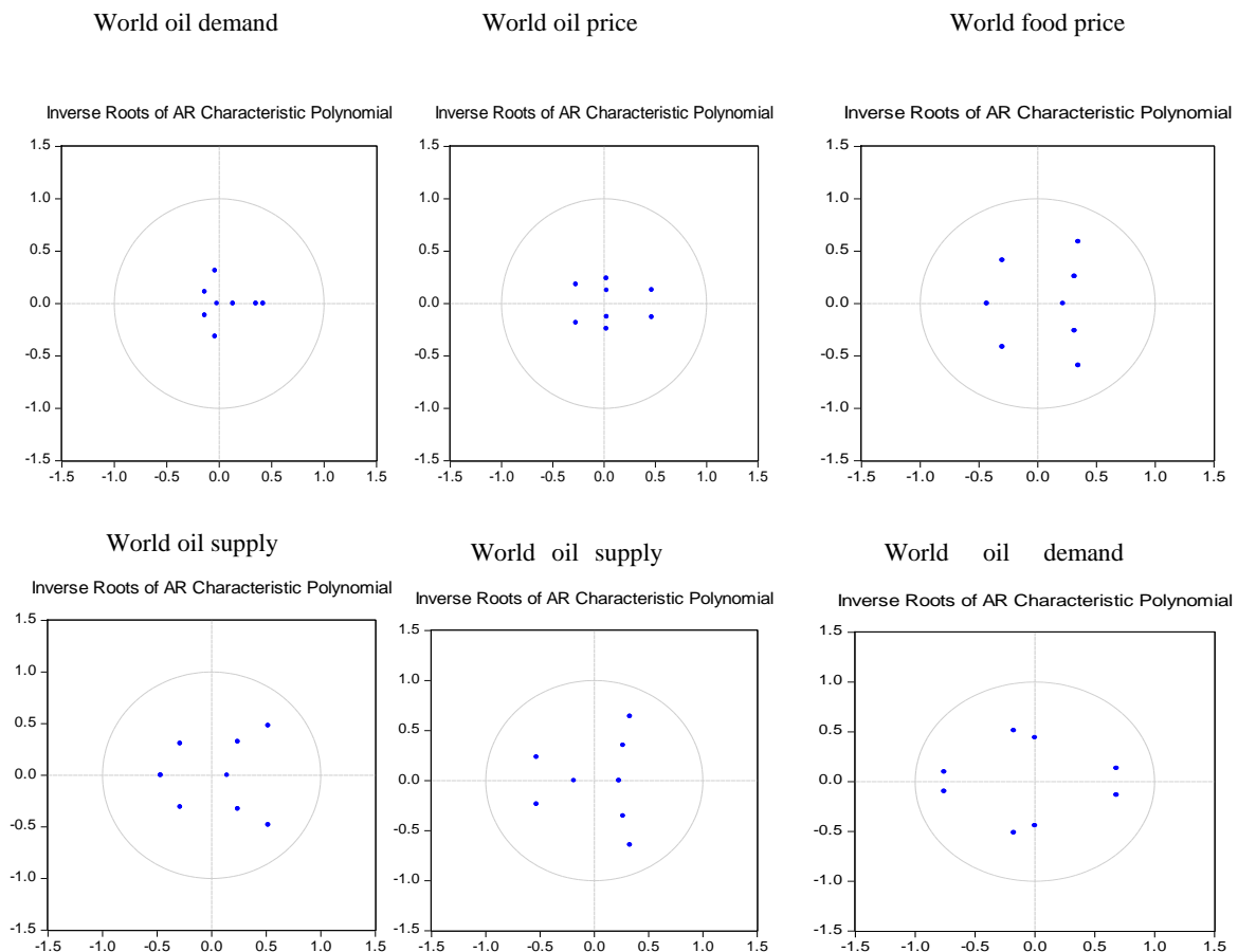
Figure 6.18: Roots test
