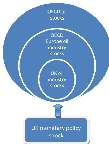
Figure 5.8: Inventory channel
