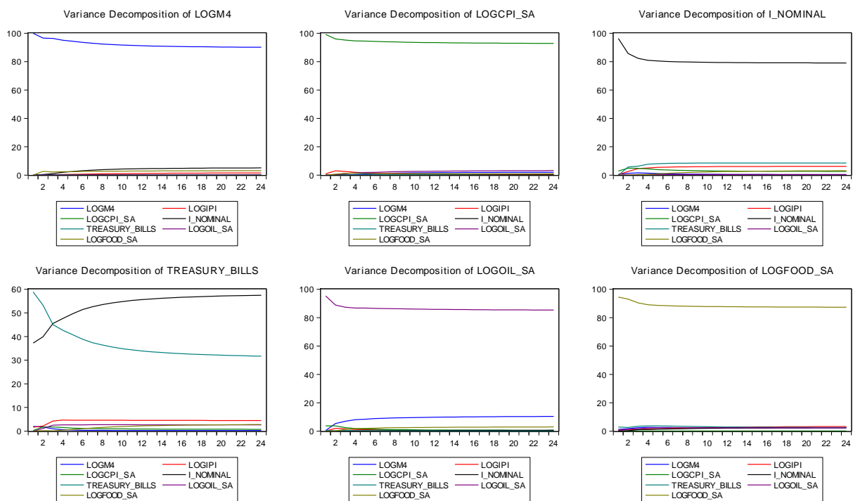
Figure 5.4: Variance decomposition
