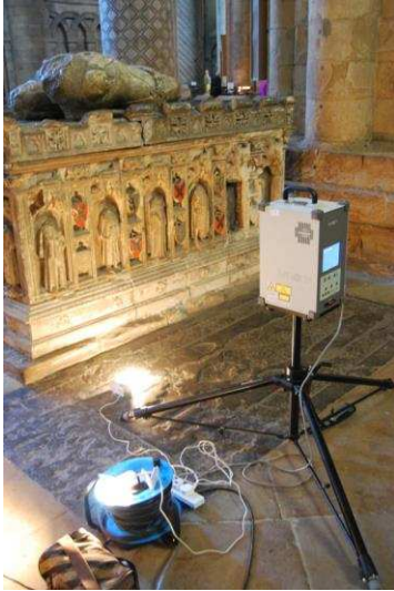
Figure 38: The Minolta 3D Scanner used to scan the surface topology of the tomb of Sir John Neville
