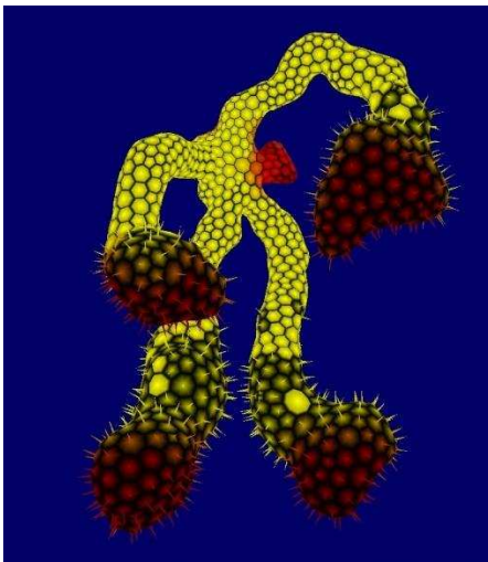
Figure 28: Kenneth Snelson 'C60'
