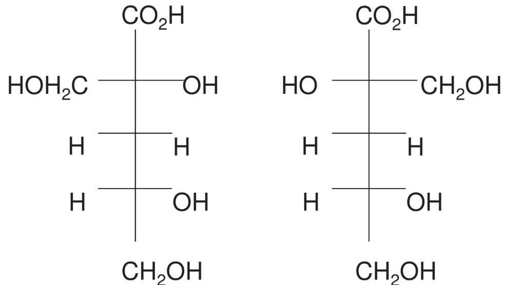
Fig 2. The \alpha - (L) and \beta - (R) conformations of isosaccharinic acid (ISA). Although the presence of ISA is not observed in the natural environment, previous research has shown that micro-organisms from neutral sediments are capable of the utilisation of both \alpha and \beta ISA within microcosm experiments. No significant difference in ISA degradation rates were observed across microcosms operating under iron reducing, sulphate reducing and methanogenic conditions at pH 7.5 [10]. When methanogenic sediments were subjected to further increases in pH (up to pH 10), the overall ISA degradation rate was slower. In addition, a difference was seen in the degradation rates of \alpha and \beta ISA suggesting the potential for the persistence of the \beta stereoisomer within and surrounding the chemically disturbed zone of an ILW-GDF [11]. These communities were incapable of surviving at a pH of 11.0, suggesting that longer timescales may be required for micro-organisms to adapt to environmental pH values above pH 10.0, rather than adapting an ability to degrade ISA. In view of this, the hyper alkaline environment present at Harpur Hill provides an alkaliphilic soil dwelling microbial consortia which may be more indicative of the consortia that may develop with the near-field of an ILW-GDF.
