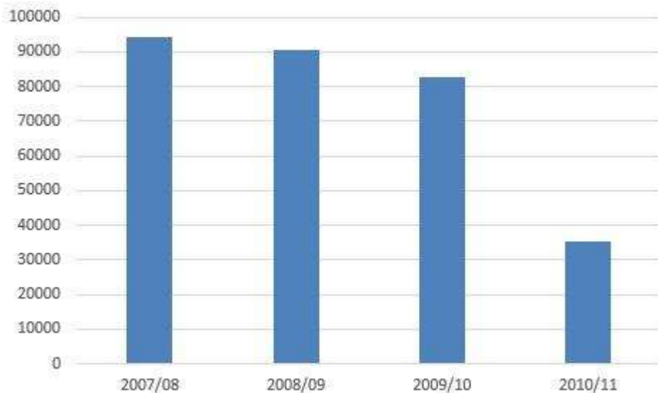
Figure 8. A&I database
