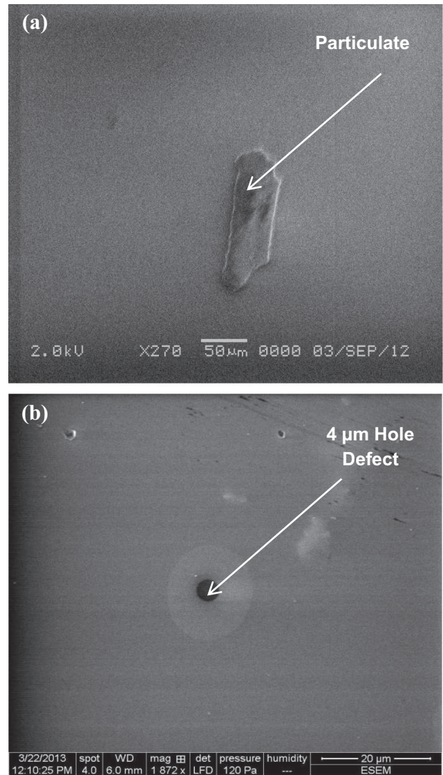
Fig. 5. Shows (a) particulate type defect, (b) hole type defect in the \text{Al}_2\text{O}_3 barrier coating (ESEM images).
