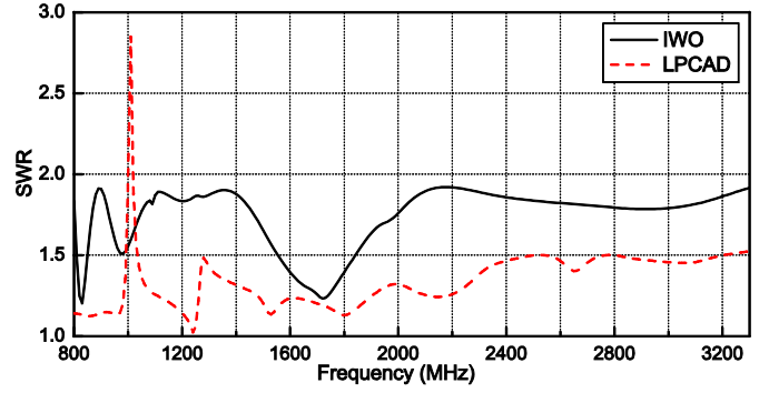
Fig. 2. SWR vs. frequency.
