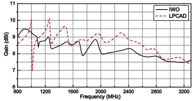
Fig. 3. Gain vs. frequency.
