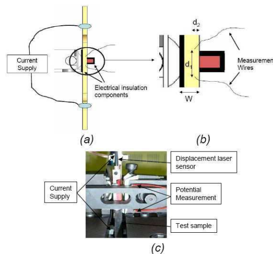
Figure 8: Schematic of the experimental set-up: (a) positioning of the current supply and isolation, (b) positioning of the measurement wires, (c) picture of the experimental set-up.
