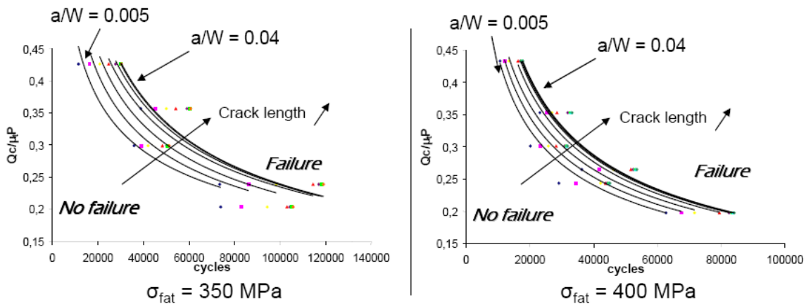
Figure 19: Evolution of the tangential crack nucleation threshold for different crack lengths.
