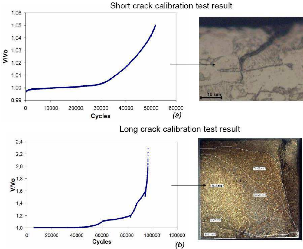
Figure 9: (a) Typical curve V = f(N) : test stopped at V/V_0 = 1,05 , \sigma_{\text{fat}} = 400 MPa and Q^*/\mu_t P = \pm 0.29 and corresponding observation, (b) Typical curve V = f(N) for a long crack calibration test: \sigma_{\text{fat}} = 400 MPa with four conditions changes during one test and corresponding observations.
