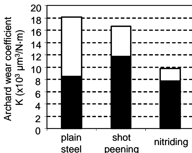
Figure 11 : Wear kinetics of the tribosystems under investigation: \square : K_{52100cylinder} counterbody; \blacksquare : K_{TREAT} , rectangular prism made of the reference steel after different surface treatments; \square + \blacksquare : K_{TOTAL} total volume wear of the fretting couple.
