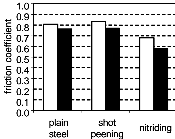
Figure 8 : Mean friction coefficients reckoned with use of incremental sliding analysis : □ friction coefficient \mu_t defined at the displacement amplitude \delta_t ; ■ friction coefficient under stabilized gross slip conditions ( \mu_{GS} ).
