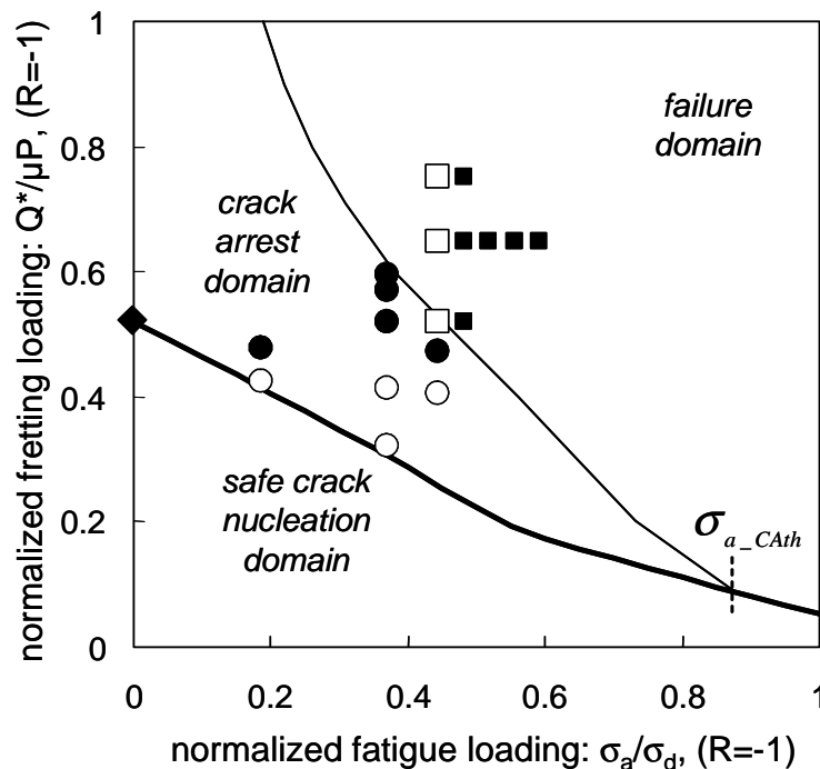
Figure 16 : Fretting-Fatigue map of the AISI 1034 steel ( p_{0H} = 450 MPa, a_H = 320 \mu m, \mu_t = 0.85 ): \circ : no crack nucleation ( 10^6 cycles); \bullet : crack nucleation ( 10^6 cycles); \blacklozenge : crack nucleation threshold identified for plain fretting conditions ( 10^6 cycles); \blacksquare : broken specimen ( 10^7 cycles); \square : unbroken specimen ( 10^7 cycles); \text{—} : theoretical crack nucleation boundary (Crossland, \ell_{3D} = 45 \mu m); \text{—} : theoretical crack arrest boundary (El Haddad's-short crack arrest methodology using friction free mixed-mode approximation).
