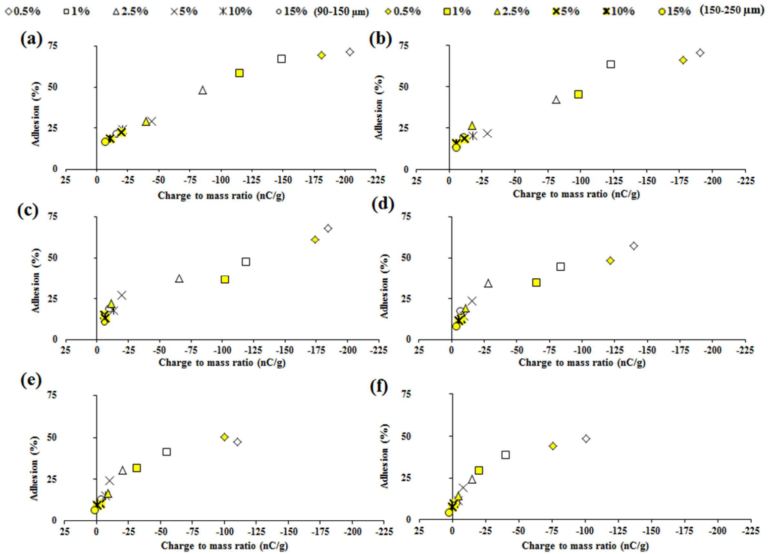
Figure 5. Effect of tribo-electric charge (nC/g) on surface adhesion (%), (a) A4M (b) F4M (c) E4M (d) K4M (e) K15M (f) K100M having polymer particle size 90-150 μm and 150-250 μm.
