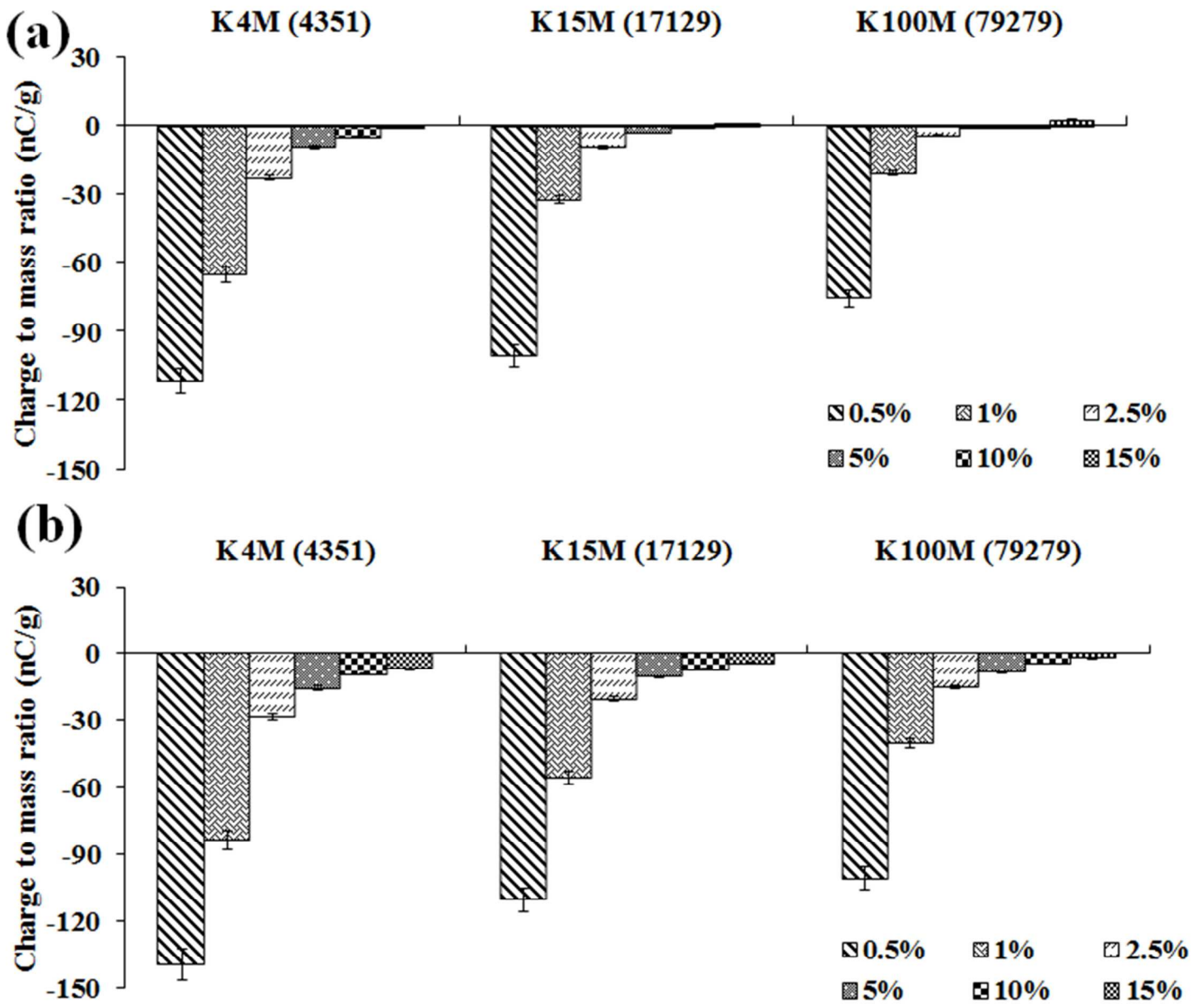
Figure 4. Effect of polymer molecular size (viscosity) on the tribo-electric charging of flurbiprofen:cellulose ether powder mixtures; polymer particle size (a) 150 - 250 \mu\text{m} and (b) 90 - 150 \mu\text{m} , n=3 , ( viscosity (cp) in parentheses on x-axis)
