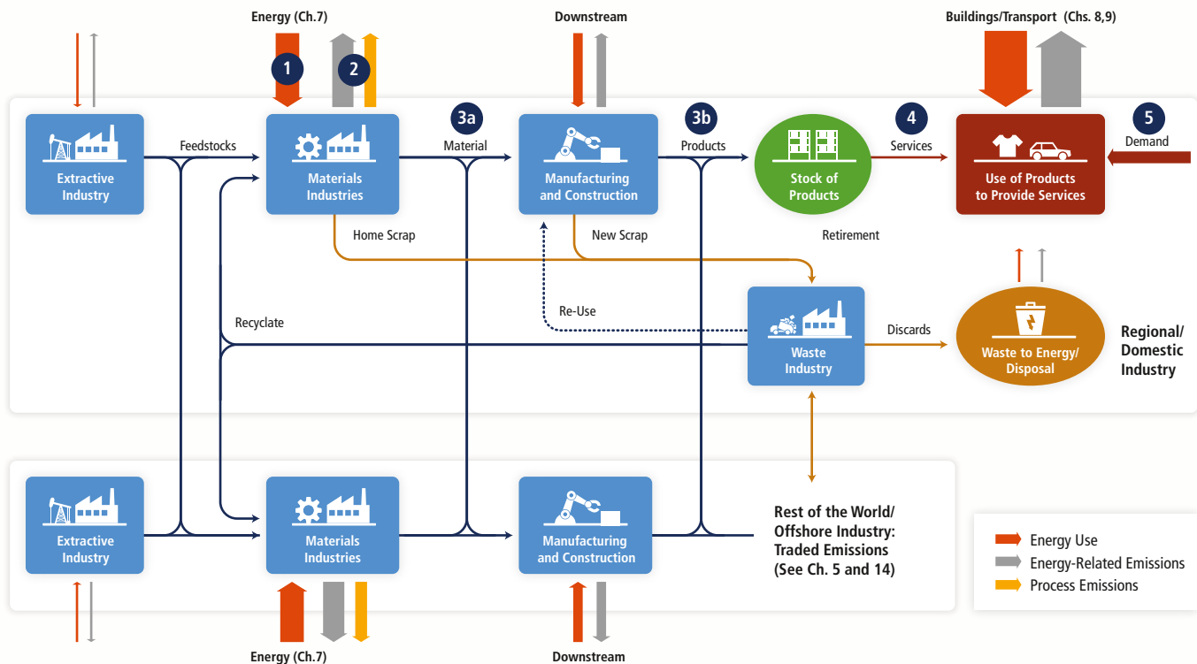
Figure 10.2 | A schematic illustration of industrial activity over the supply chain. Options for climate change mitigation in the industry sector are indicated by the circled numbers: (1) Energy efficiency (e.g., through furnace insulation, process coupling, or increased material recycling); (2) Emissions efficiency (e.g., from switching to non-fossil fuel electricity supply, or applying CCS to cement kilns); (3a) Material efficiency in manufacturing (e.g., through reducing yield losses in blanking and stamping sheet metal or re-using old structural steel without melting); (3b) Material efficiency in product design (e.g., through extended product life, light-weight design, or de-materialization); (4) Product-Service efficiency (e.g., through car sharing, or higher building occupancy); (5) Service demand reduction (e.g., switching from private to public transport).
