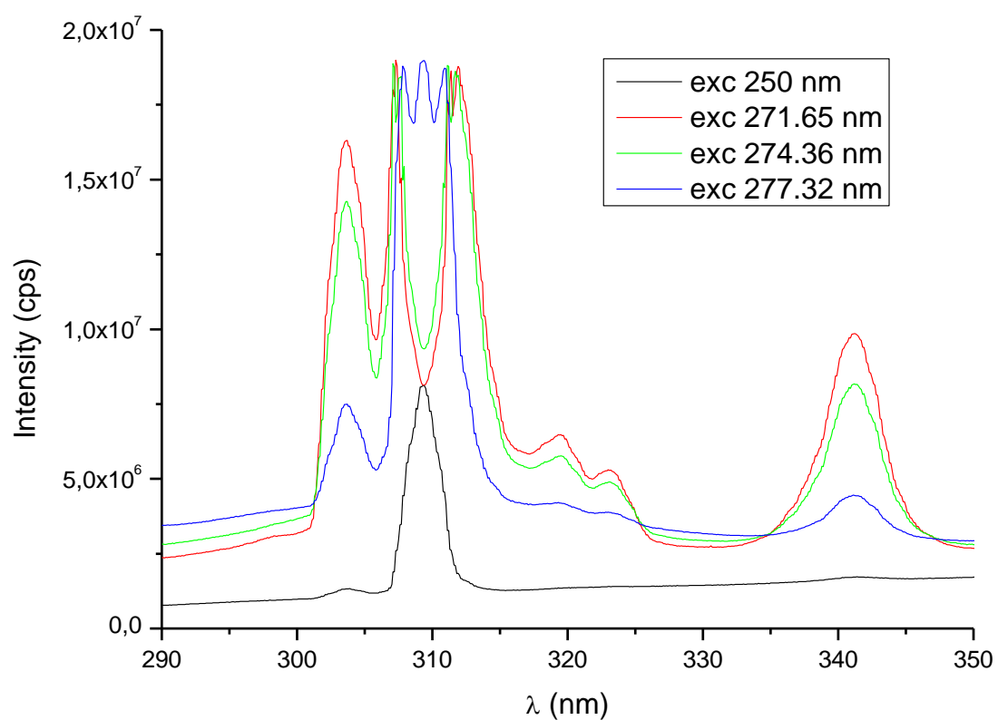
Figure 7.6 Emission spectra of Gd 2 O 3 nanoparticles. Spectra were recorded by visiting PhD student Maria Gomes in the Corr Group. The excitation wavelengths used were 250 nm, 271.65 nm, 274.36 nm and 277.32 nm.
