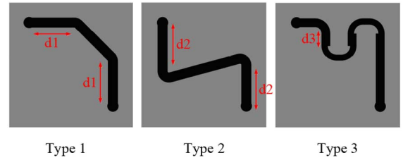
Fig. 16. Three types of microstrip phase delay lines employed in the passive reflectarray demonstrators.
