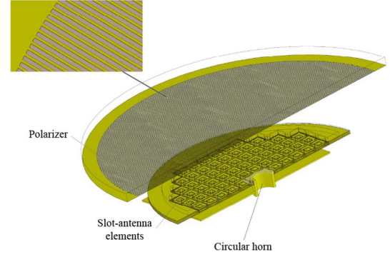
Fig. 15. 3-D sectional view of the folded reflectarray.
