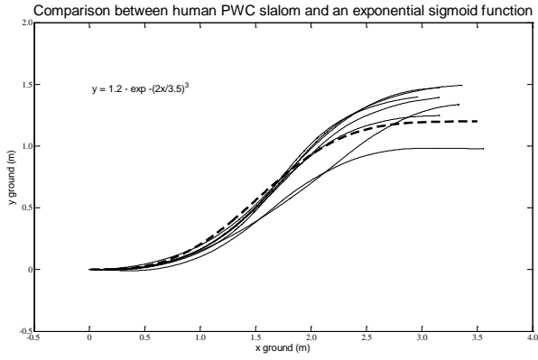
Fig. 5. Exponential sigmoid compared with human trajectories
