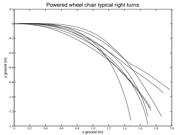
Fig. 3. Human turn PWC trajectories
