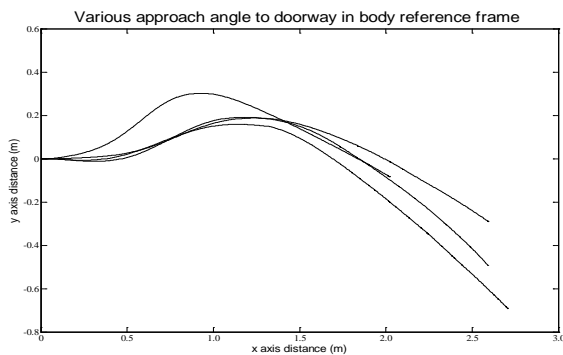
Fig. 10. Generated trajectory with DLAFF collision avoidance in an autonomous mode
