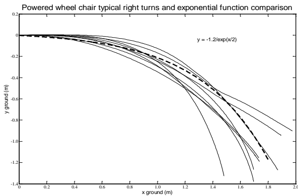
Fig. 6. Exponential curve compared with human turn trajectories
