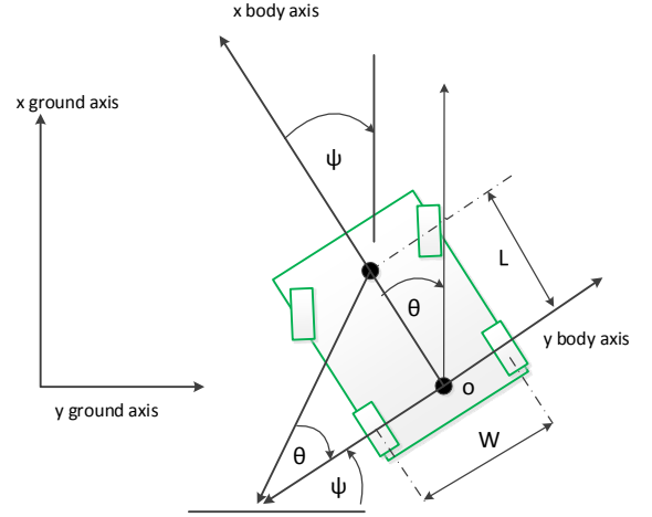
Fig. 1. Robotic platform frame of reference and kinematic
