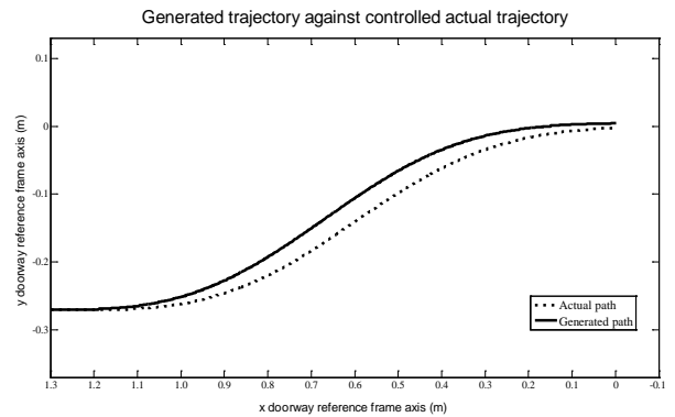
Fig. 8. System generated trajectory and actual path platform took with the operator-in-the-loop
