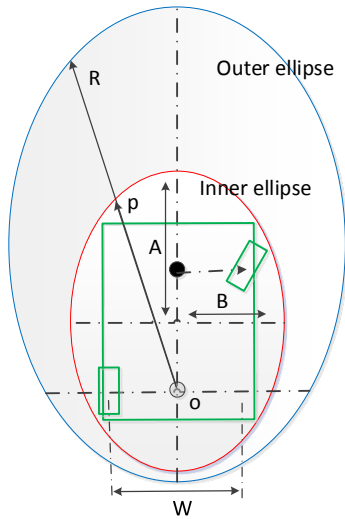
Fig. 7. Elliptical obstacle avoidance model
