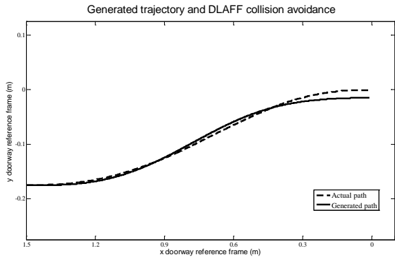
Fig. 9. Generated trajectory with DLAFF collision avoidance with the operator-in-the-loop
