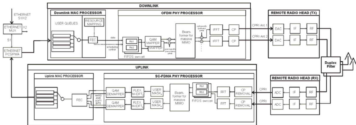
Fig. 7 The beamforming operation for massive MIMO can be shifted from the BBU/CO to the RRH in order to reduce the data rate in the fronthaul.
