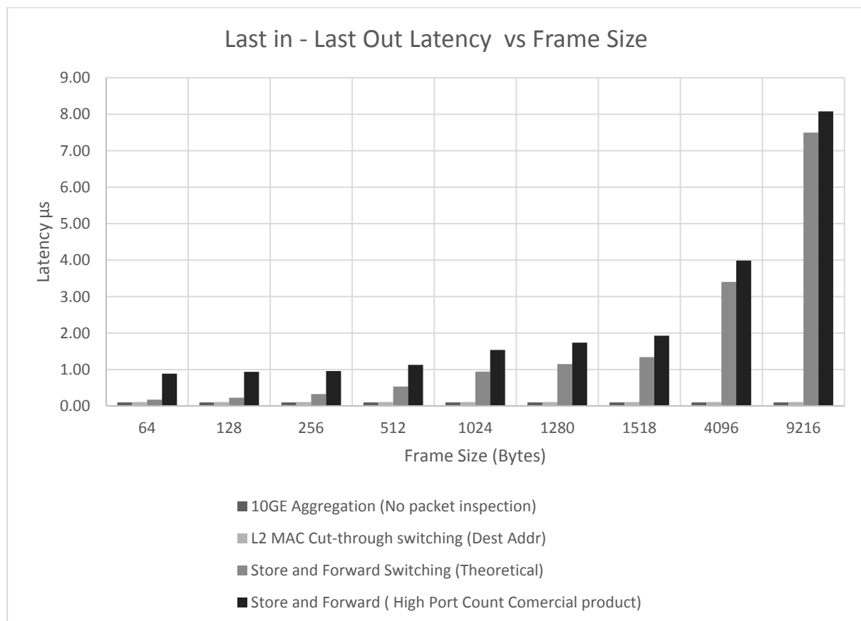
Figure 5 Last bit in to last bit out latency for cut-through and store-and-forward Ethernet switching (one-way, uncontended packets)
