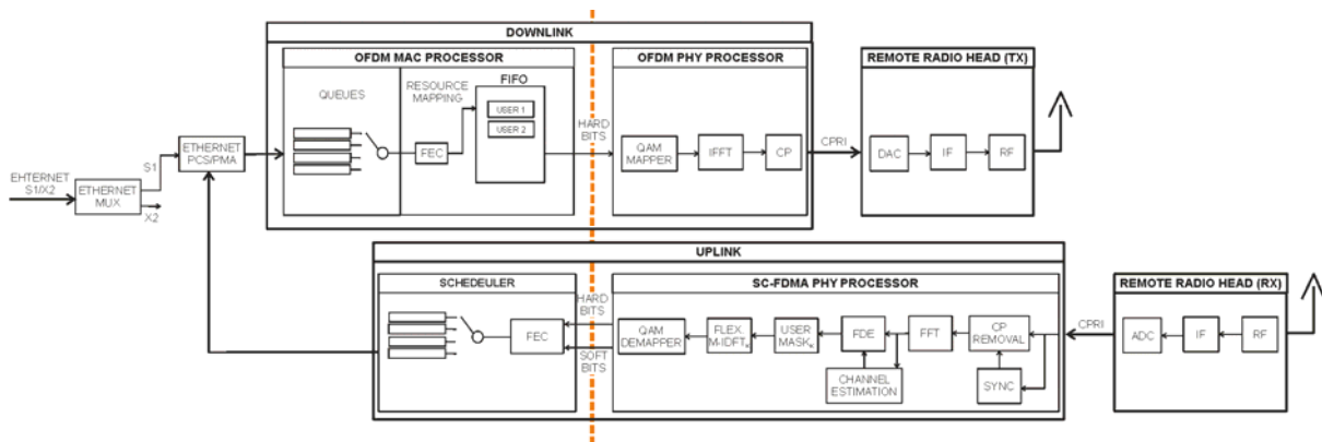
Fig. 6 Signal processing in an LTE base station.
