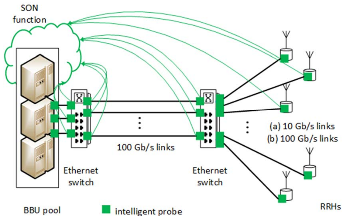
Figure 3 – BBU pool connected to RRHs through Ethernet switches. In option (a), lower-speed links are used beyond an aggregation point that may make use of statistical multiplexing gains. In option (b), the links have the same line rate, permitting the use of cut-through operation.
