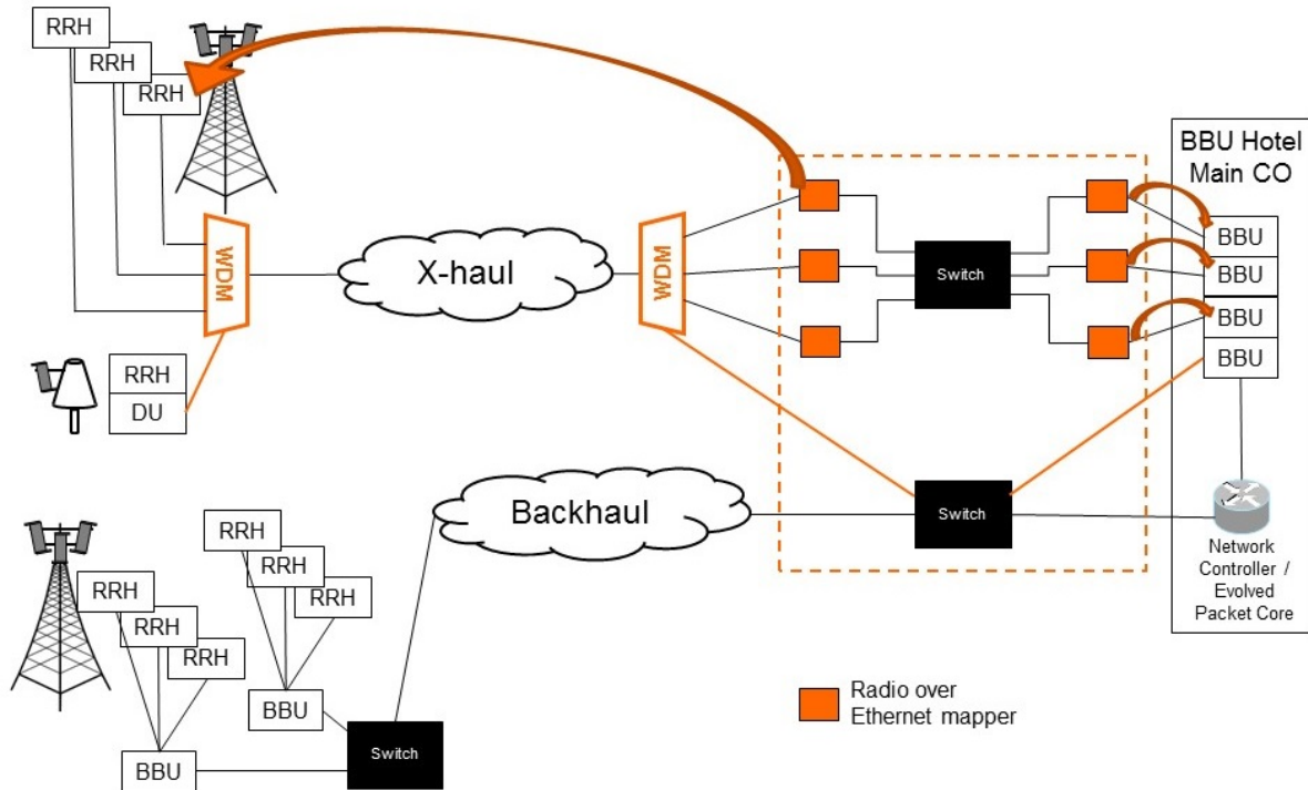
Figure 9: Global picture of Ethernet based network including back- and front-haul
