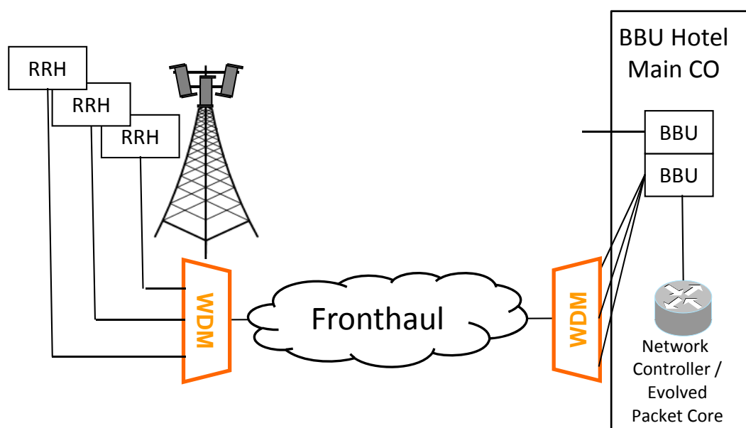
Figure 4 Fronthaul network based on WDM (Wavelength Division Multiplexing)
