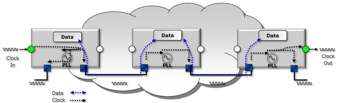
Figure 2 Synchronous Ethernet operation: clock extraction and resynchronization is carried out at each node
