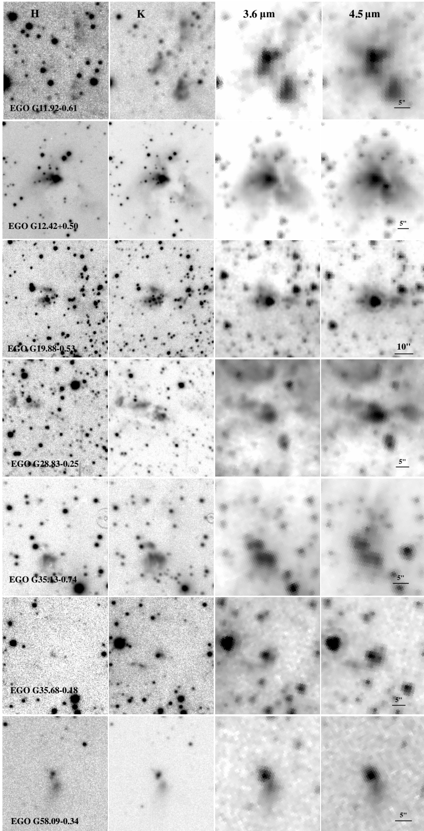
Fig. 25.— EGOs with H -band emission; H , K , 3.6 \mu\text{m} , and 4.5 \mu\text{m} images in the first, second, third, and fourth columns, respectively.
