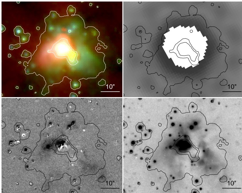
Fig. 5.— Same as Figure 1, but for EGO G12.42+0.50. The white part in the 24 \mu\text{m} source is saturated.
