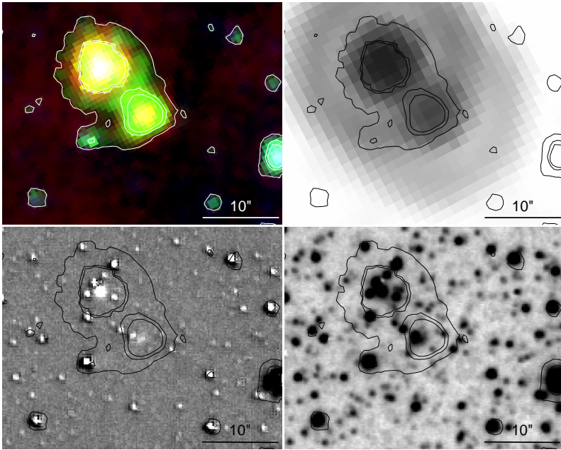
Fig. 12.— Same as Figure 1, but for EGO G20.24+0.07.
