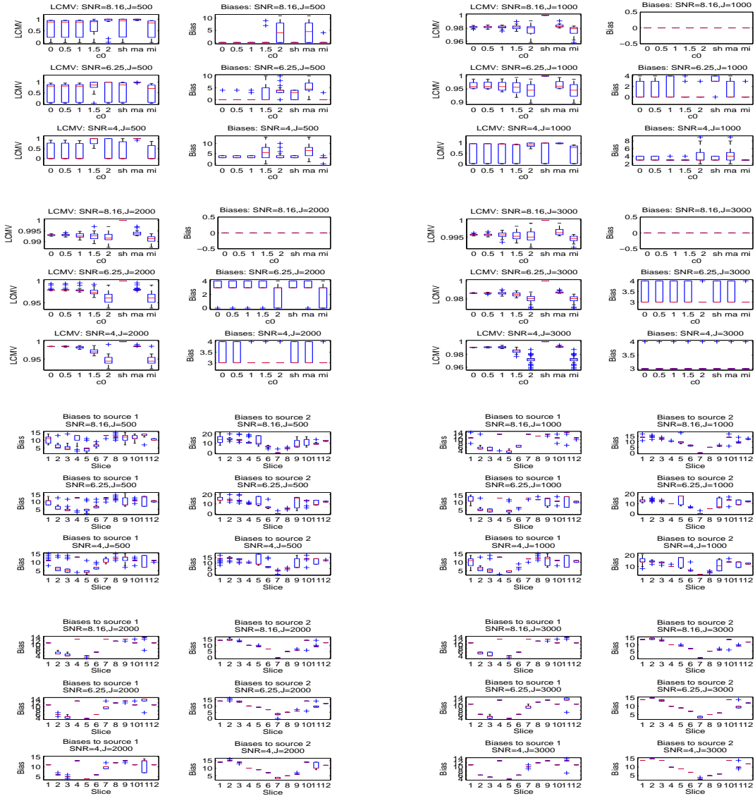
Figure 4: Scenario 3: Two sources located at CTF coordinates (3, -1, 4)^T cm and (-5, 2, 6)^T cm respectively. The first six rows show the box-and-whisker plots of the index values and the localization biases against the tuning constant c_0 = 0, 0.5, 1, 1.5, 2, \mathbf{ma}, \mathbf{mi} and \mathbf{sh} for the combinations of n = 102 sensors, \text{SNR} = 1/0.35^2, 1/0.4^2, 1/0.5^2 , and the sample rates J = 500, 1000, 2000, 3000 respectively. The last six rows give the box-and-whisker plots of the minimum local localization bias to the sources r_1 and r_2 against the transverse slice indices from 0 to 10 when c_0 is selected by the minimum strategy for these combinations respectively. The red colored lines in the boxes are the medians. When the upper and lower quartiles and medians of localization biases are equal, the box in the plot will reduce to a red colored line. The last six rows of the plots show all the local peaks among the transverse slices are not close to the source location r_1 , implying the source 1 has been masked on the neuronal activity map by source cancellations.
