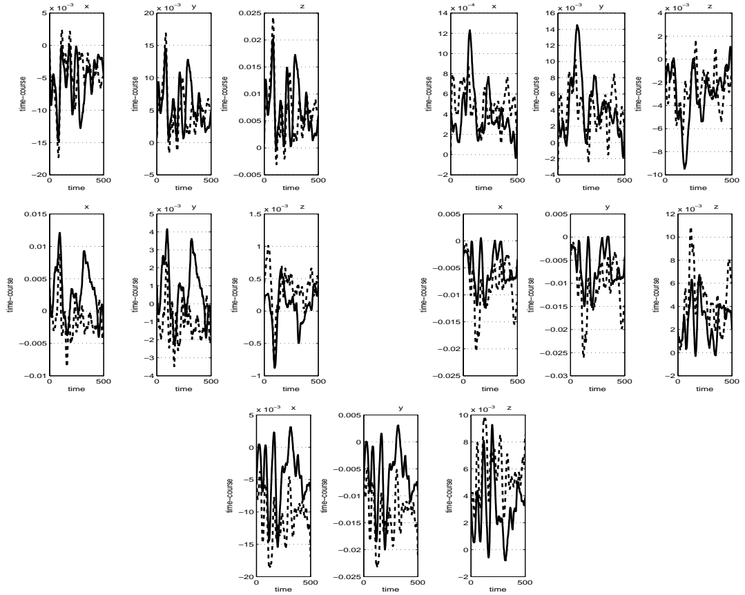
Figure 12: Plots of the estimated time-courses at the global peaks along x , y and z -axes respectively for each of five sessions. The solid curve and the dashed curve in each plot stand for the estimated time-courses under the faces and the scrambled faces respectively. The plots are ordered from the top left panel to the right panel to the bottom panel corresponding to sessions 1 \sim 5.
