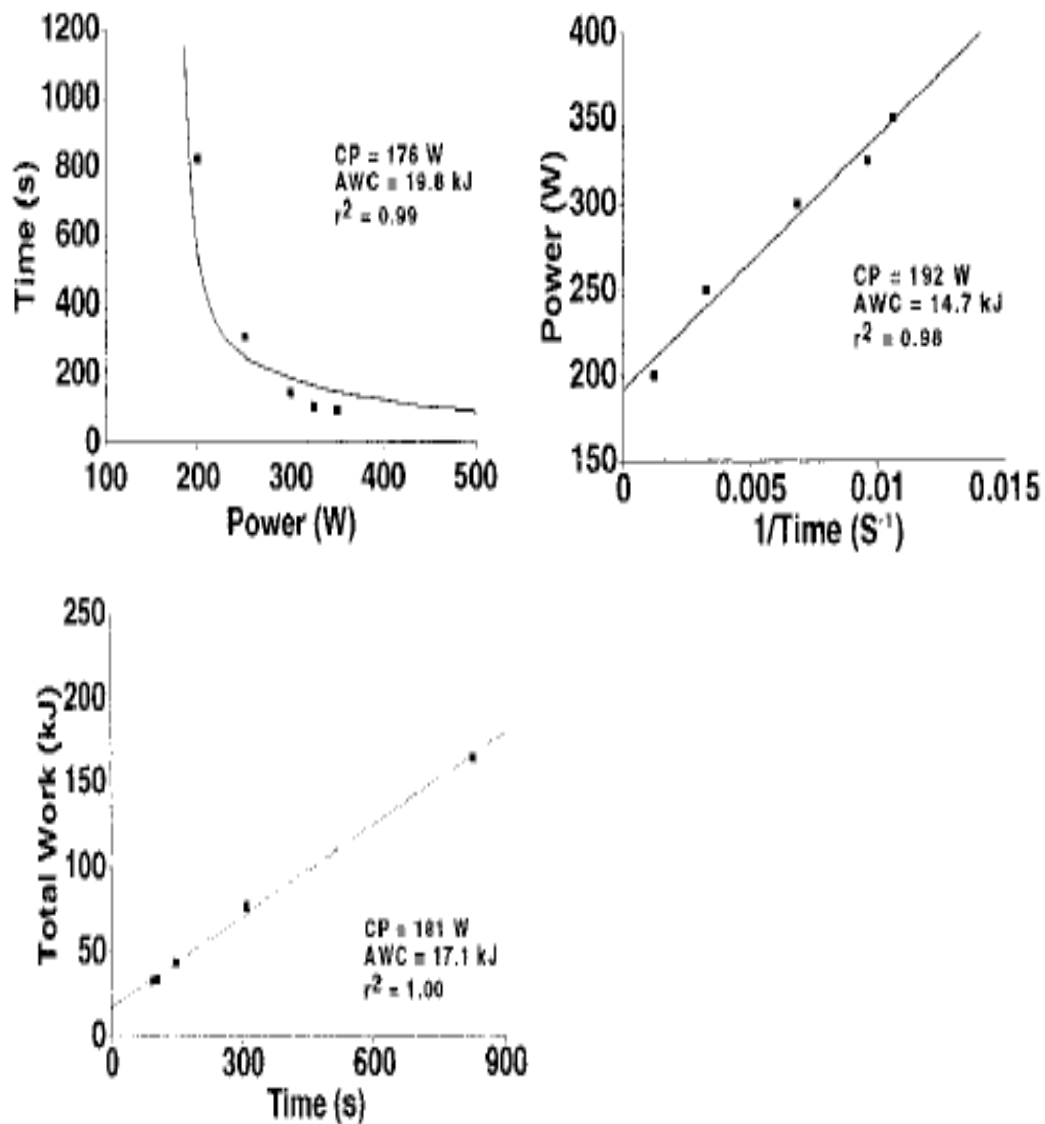
Figure 2.2. The three models presented graphically. (Bull et al., 2000, p.527).
