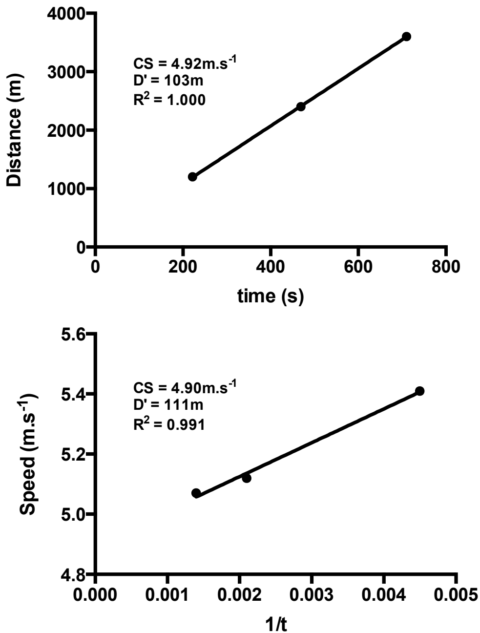
Figure 4.1: Data plots from a representative subject showing the CS, D' and R^2 calculated from the linear distance-time model (top) and inverse of time model (bottom). Data are modelled using the values from subject 1, trial 1.
