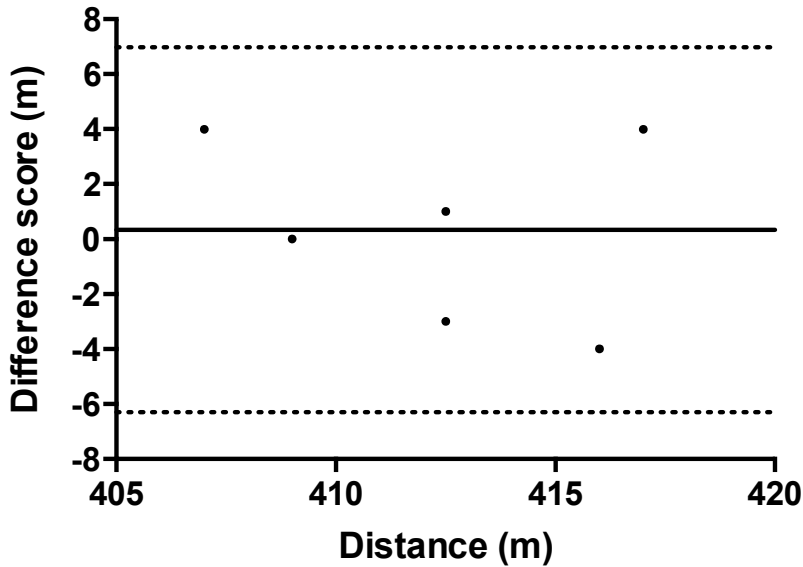
Figure 3.1: Bland-Altman plot of the agreement between actual distance and Garmin recorded distance between repeated trials within the same day. The solid horizontal line represents the mean bias, whilst the dashed lines represent the 95% limits of agreement. Data are from trials 2-1.
