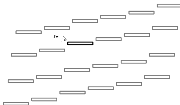
Fig.2 Skewed lattice frame dipole FSS
