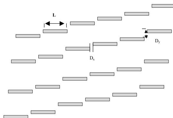
Fig.1 Skewed lattice solid dipole FSS
