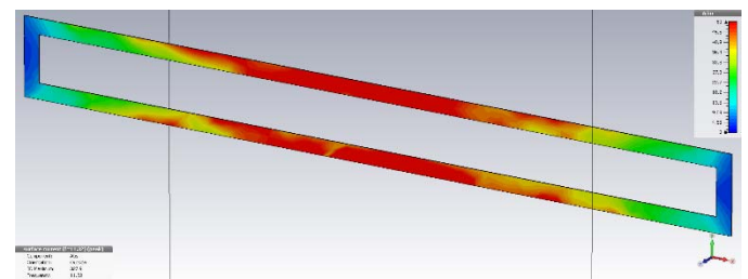
(b) Frame dipoles
