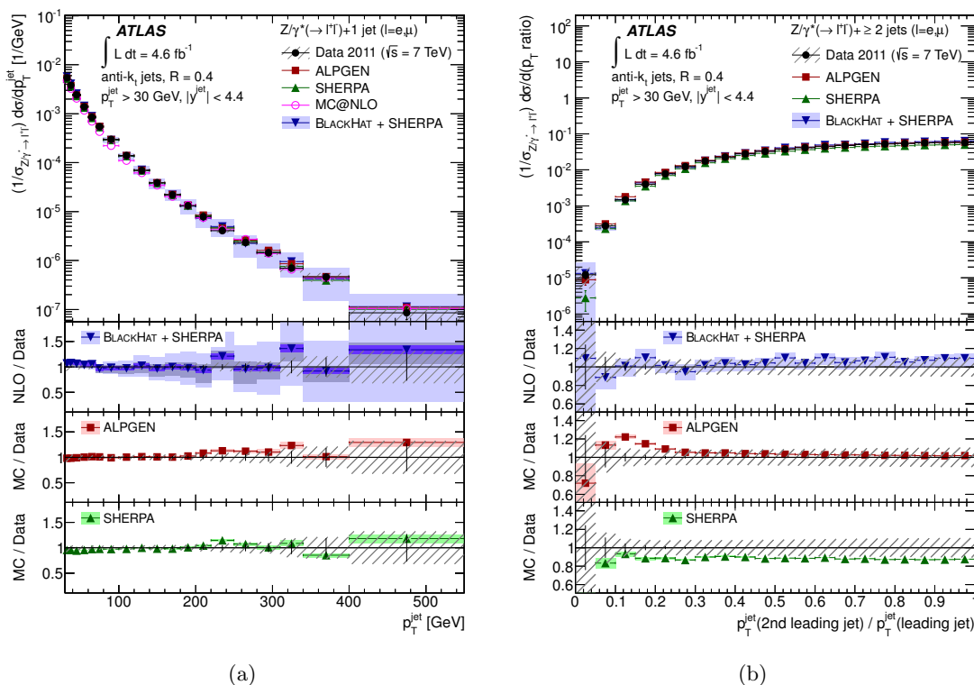
Figure 7. (a) Measured cross section for Z(\rightarrow \ell\ell) + \text{jets} as a function of the jet transverse momentum, p_T^{jet} , for events with exactly one jet with p_T^{jet} > 30 GeV and |y^{jet}| < 4.4 in the final state and (b) as a function of the ratio of p_T^{jet} of the second leading jet to p_T^{jet} of the leading jet for events with at least two jets. The cross sections are normalized to the inclusive Z(\rightarrow \ell\ell) cross section. The other details are as in figure 3.
