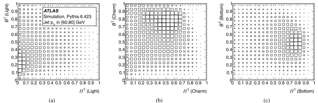
Fig. 5 Two-dimensional distributions of \Pi^\top and B^\top (flavour templates) obtained with PYTHIA 6.423 for (a) light, (b) charm and (c) bottom jets with p_T in the bin [60, 80] GeV
