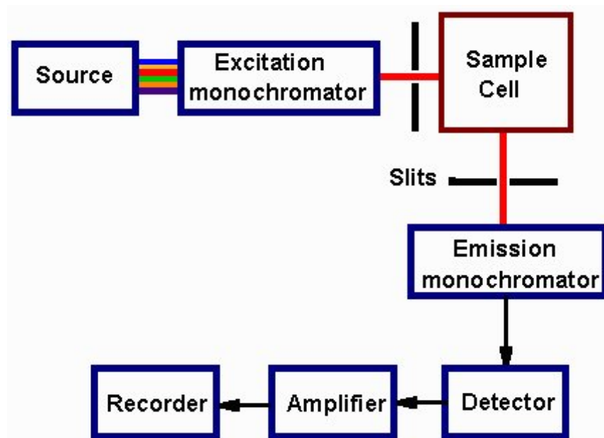
Figure 2-4: Fluorimeter schematic
