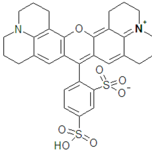
Figure 2-6: Sulforhodamine 101 structure
