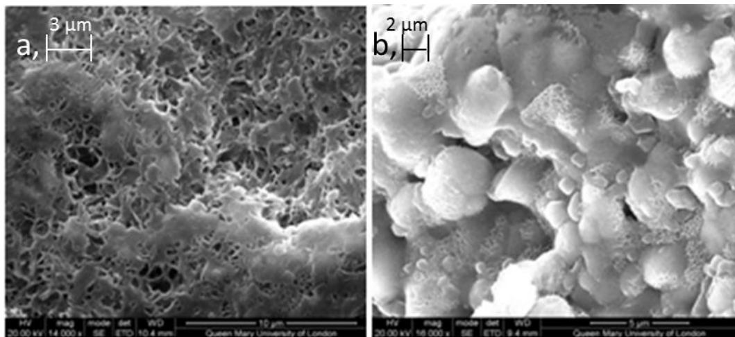
Figure 4-5: Scanning electron image showing the differences in strut porosity between (a) SAG 80/30 and (b)SAG 80/20.
