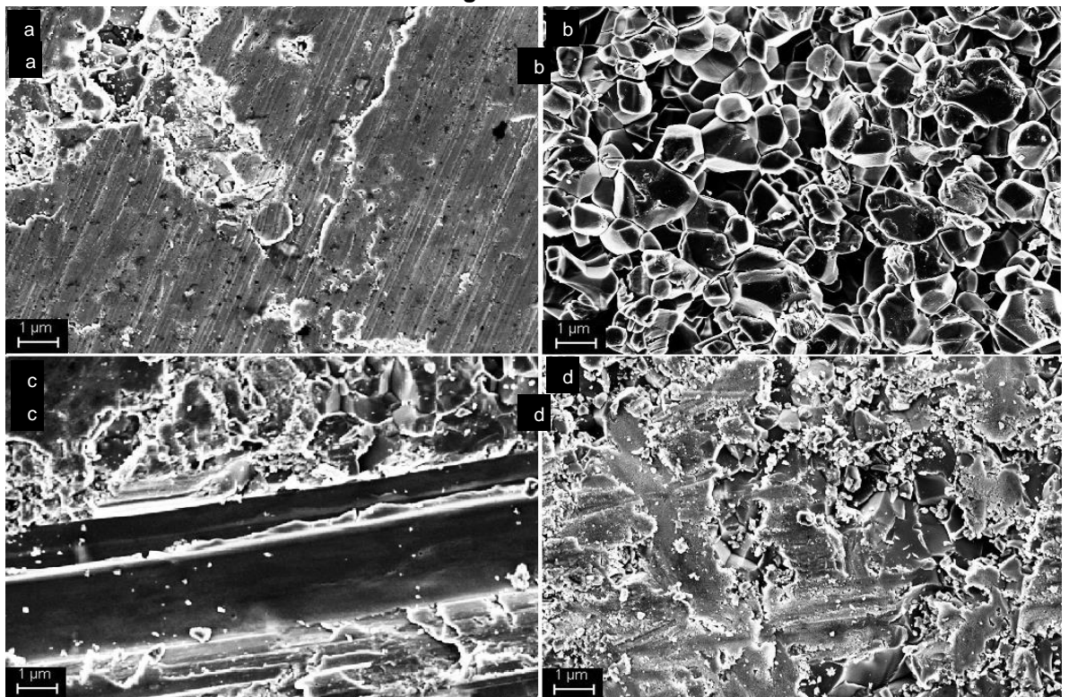
Figure 6-17: SEM images of the HA-TCP original as received (a), AE (b), 80Grit (c) and 1000Grit (d) disc surfaces at 10K magnification
