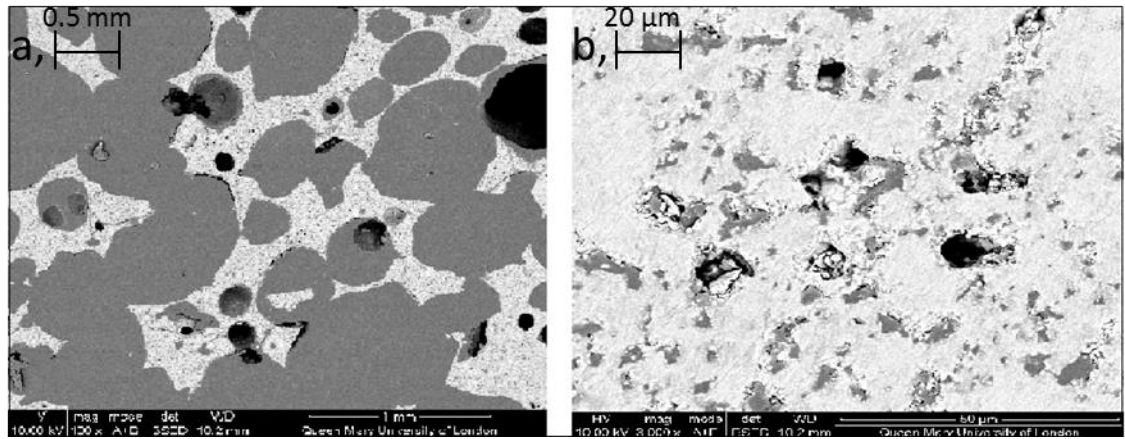
Figure 3-6: SEM images of porous HAG80/20 embedded in resin and polished used to determine the strut porosity at (a) 100 and (b) 3000 magnification
