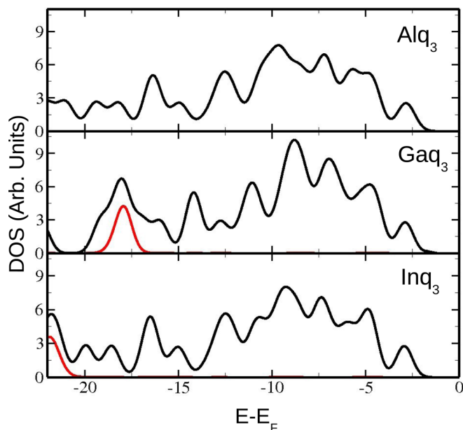
FIG. 3. (Color online) Calculated DOS (black line) for \text{Alq}_3 (top panel), \text{Gaq}_3 (middle), and \text{Inq}_3 (bottom). The red lines represent the 3d-Ga and the 4d-In states. The spectrum was rigidly displaced in order to align the HOMO at the energy corresponding to \Phi - \text{IP} (where IP is the computed ionization potential and \Phi is the experimental work function determined from the low-energy cutoff). A Gaussian broadening was added to the computed DOS in order to better compare the theoretical and the experimental spectra in Fig. 2.
