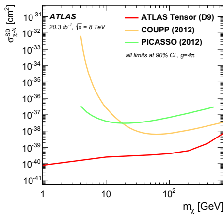
Fig. 6 Upper limits at 90 % CL on the spin-dependent \chi -nucleon cross-section ( \sigma_{\chi-N}^{SD} ) for the tensor operator D9 (red) as a function of m_\chi . The yellow and green curves represent the exclusion limits recently set by the COUPP and PICASSO collaborations [8, 9, 65]. The coupling is assumed to be g_q g_\chi = g = 4\pi
