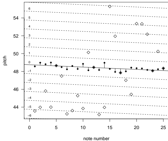
FIG. 4: Example of pitch error estimation, showing pitch measurements p_i (empty bullets) and local tonic estimates t_i (filled) using a linear fit. The stems represent the pitch error e_i .
