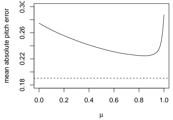
FIG. 9: Mean absolute error for models based on Eq. (9) for different values of the memory weight \mu . An optimum is recognisable around \mu = 0.85 . Dashed line: best linear prediction.
