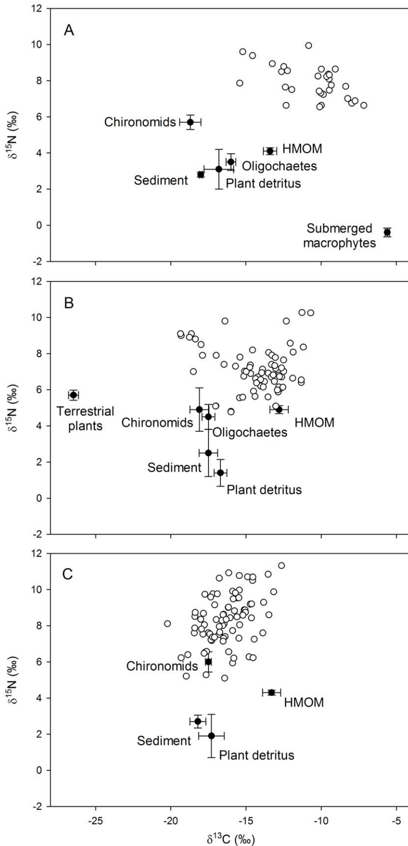
Figure 1. Stable isotope bi-plots of the Lake Naivasha food web derived from samples collected during July in A) 2001, B) 2002, and C) 2003. Open symbols represent individual Procamburus clarkii relative to the putative basal resources (solid symbols: means \pm SE from n=5 to 15) which were present and sufficiently abundant during collection to be analysed for stable isotopes. HMOM – Hippo Mediated Organic Matter. doi:10.1371/journal.pone.0042575.g001
