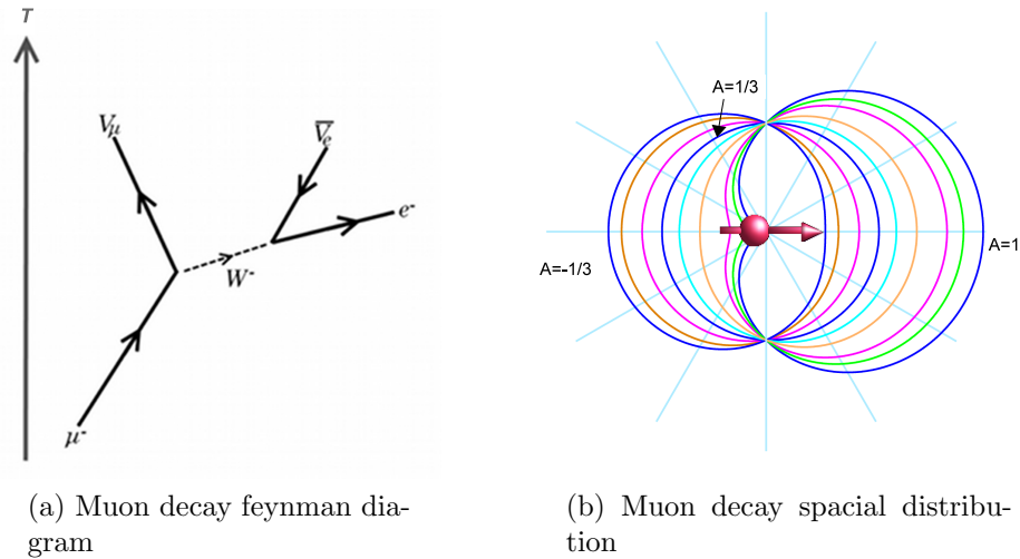
Figure 4.7: Muon decay
