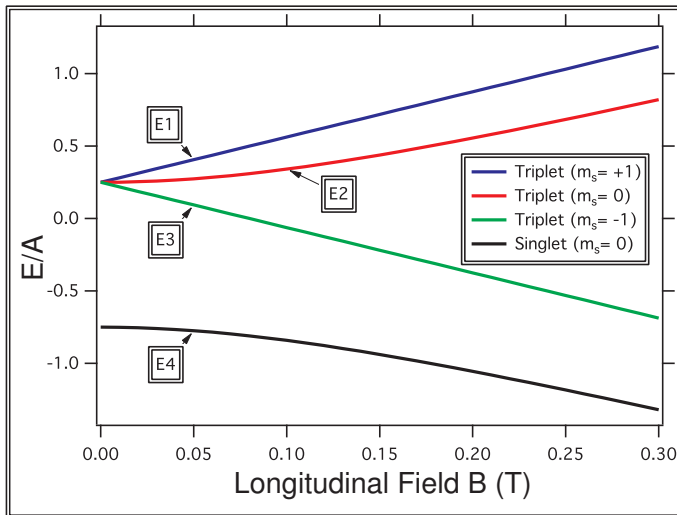
Figure 5.1: Energy levels of isolated muonium as a function of LF
