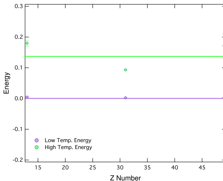
Figure 9.4: Z-dependance of the energies in the Quinolinate series
