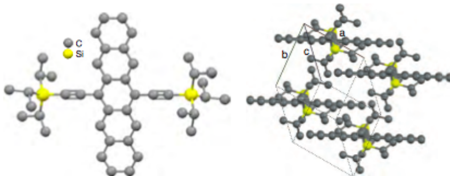
Figure 3.5: TIPS-Pentacene molecule and crystal structure
