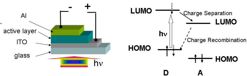
Figure 2.3: Organic solar cell
