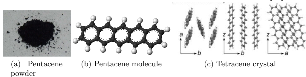
Figure 3.3: Pentacene
