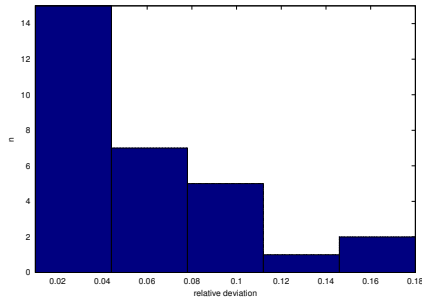
Fig. 6. The distribution of the relative deviation of the grouping algorithm.
