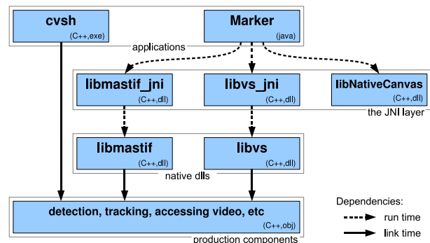
Fig. 5. The proposed architecture of the annotation system
