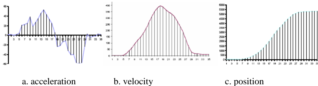
Figure 4-14; a. acceleration: actual acceleration data as obtained using an accelerometer sensor, b. velocity: velocity after single integration, c. position: distance travelled from zero after a double integration
