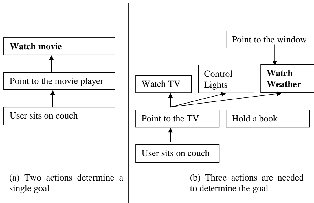
Figure 4-8: The structure of a Hierarchical Goal Determination Process based on action mapping. (a) Action maps to a single goal, (b) action maps to multiple goals until a third action is performed.
