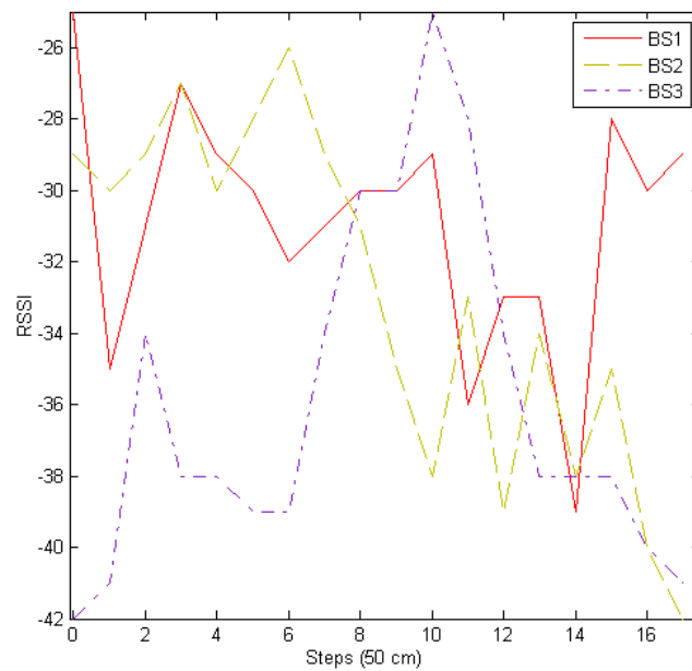
Figure 4-12: RSSI values collected from the 3 Base Stations
