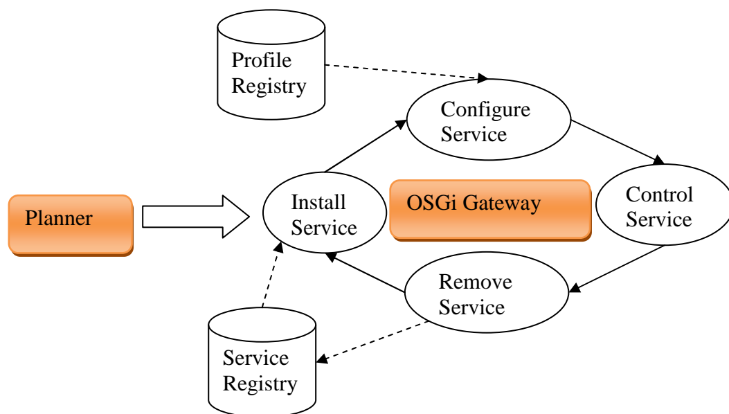
Figure 4-5: The OSGi gateway system architecture
