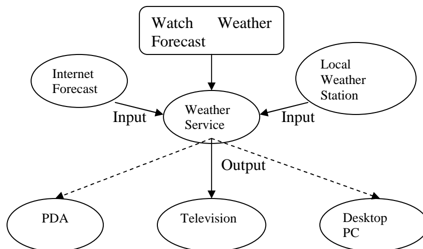
Figure 4-10: Forward chain plan for the Watch Weather Forecast goal
