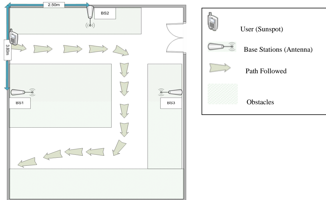
Figure 4-11: Experiment environment floor plan showing the base station position and the path followed by the Sun SPOT
