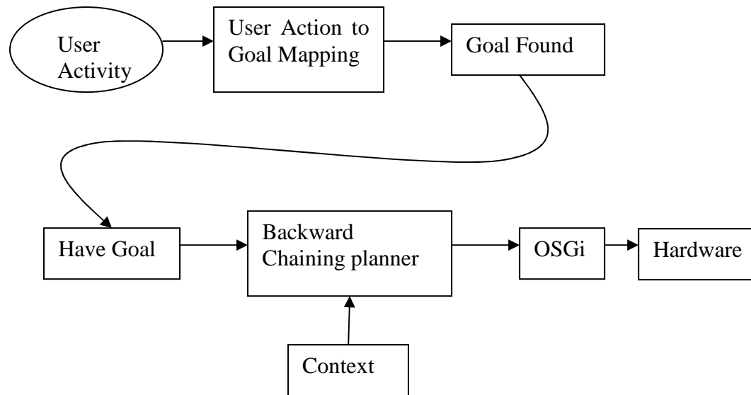
Figure 4-7: The two phases in proposed planner framework: Goal Identification and Plan Creation.
