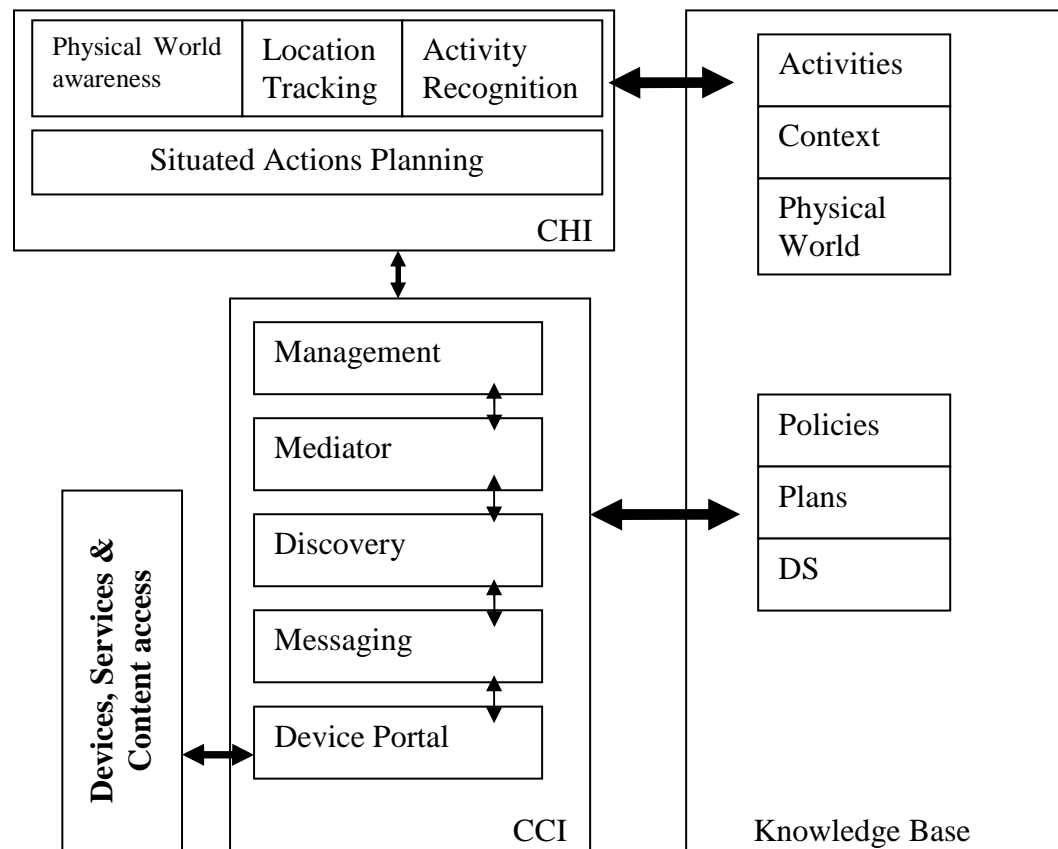
Figure 4-1: Generic System Architecture
