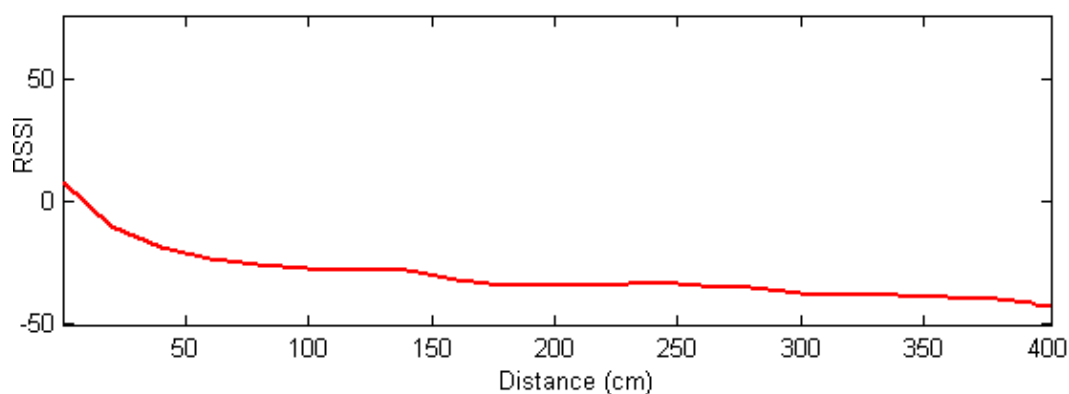
Figure 4-13: Relation between RSSI and Distance on the free space propagation model
