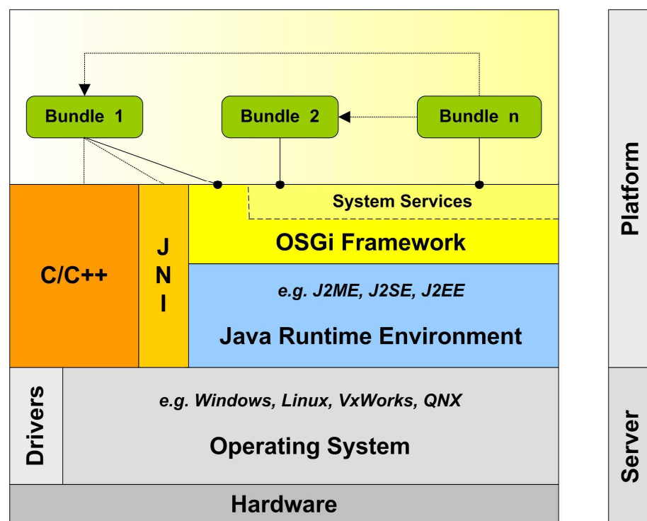
Figure 3-1: The OSGi layer specification
