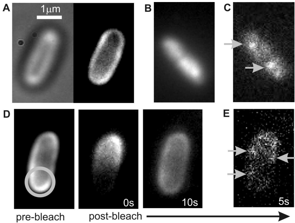
Visualisation of GFP fluorescence in E. coli YTL01 61x46mm (600 x 600 DPI)
